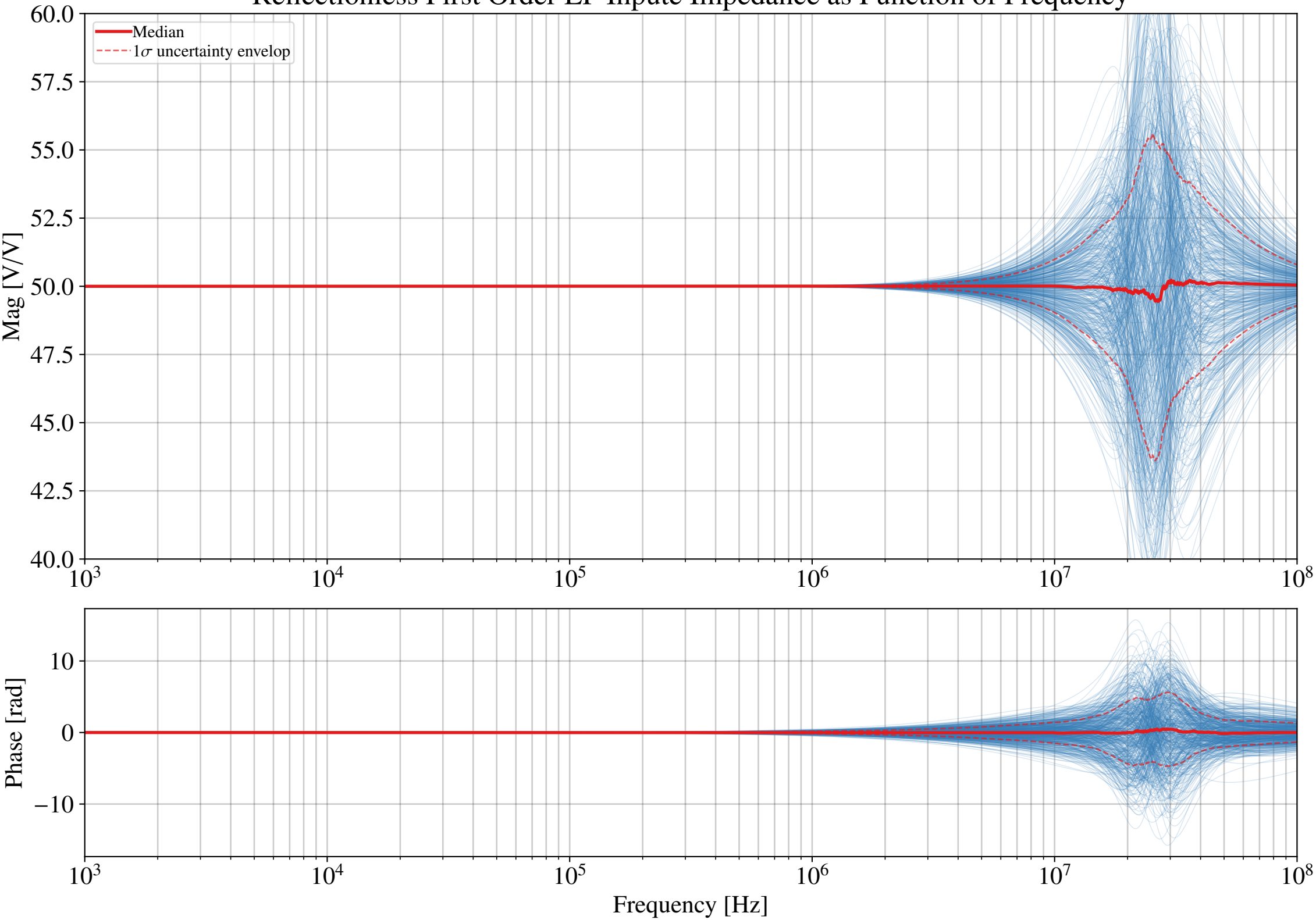
Reflectionless First Order LP Input Impedance as Function of Frequency
