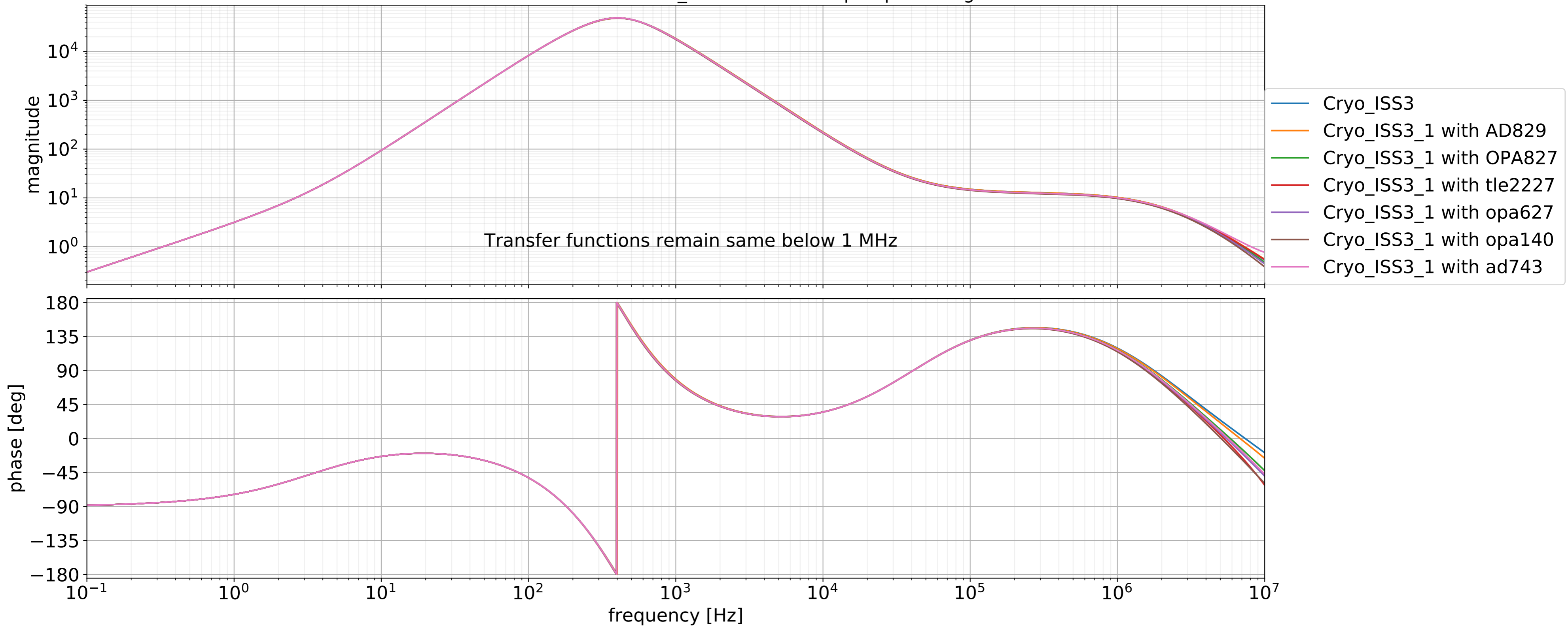
Transfer functions for ISS3 and ISS3_1 with different opamps at stage 1
