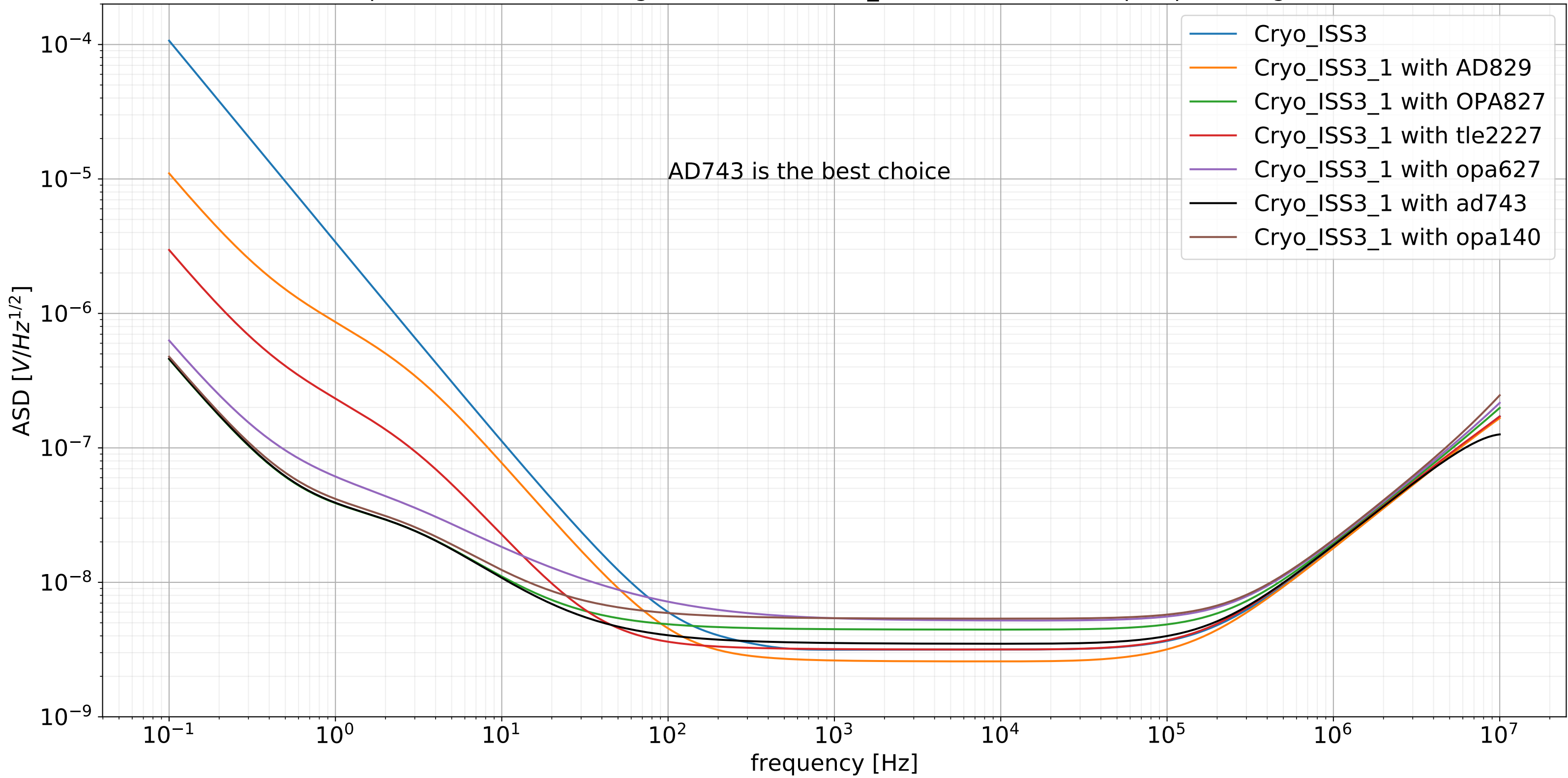
Input referred noise change from ISS3 to ISS3_1 and with different opamps at stage 1
