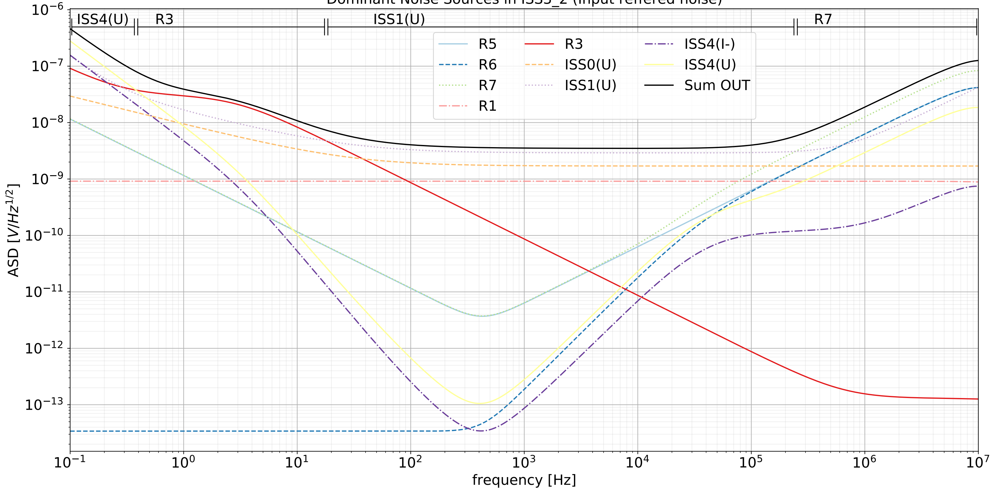
Dominant Noise Sources in ISS3_2 (Input referred noise)
