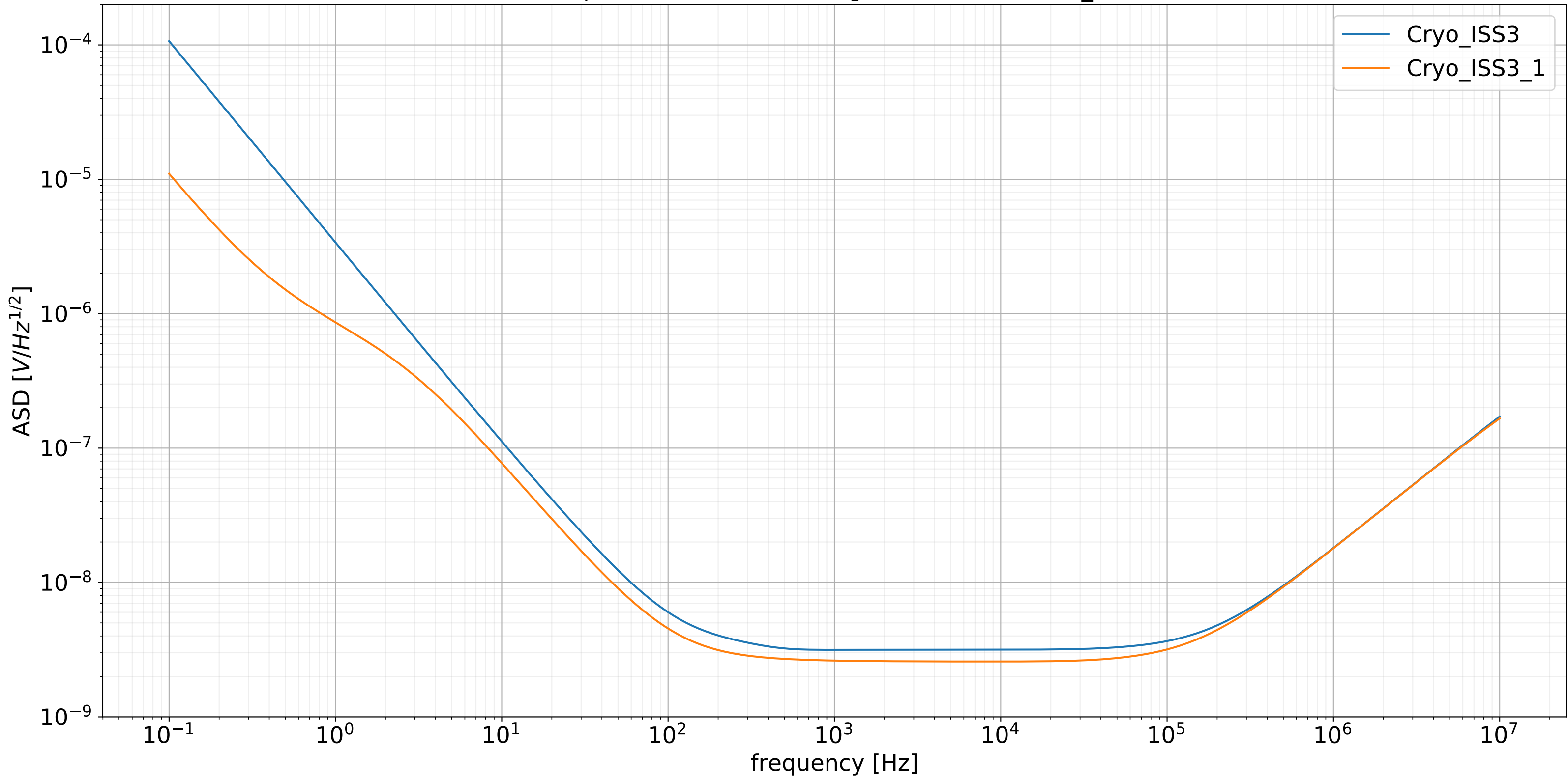
Input referred noise change from ISS3 to ISS3_1
