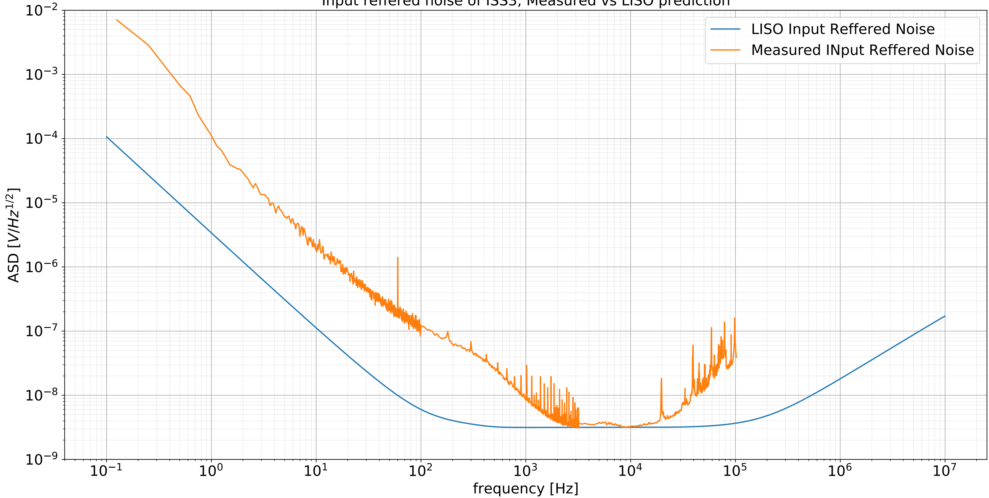
Input reffered noise of ISS3, Measured vs LISO prediction
