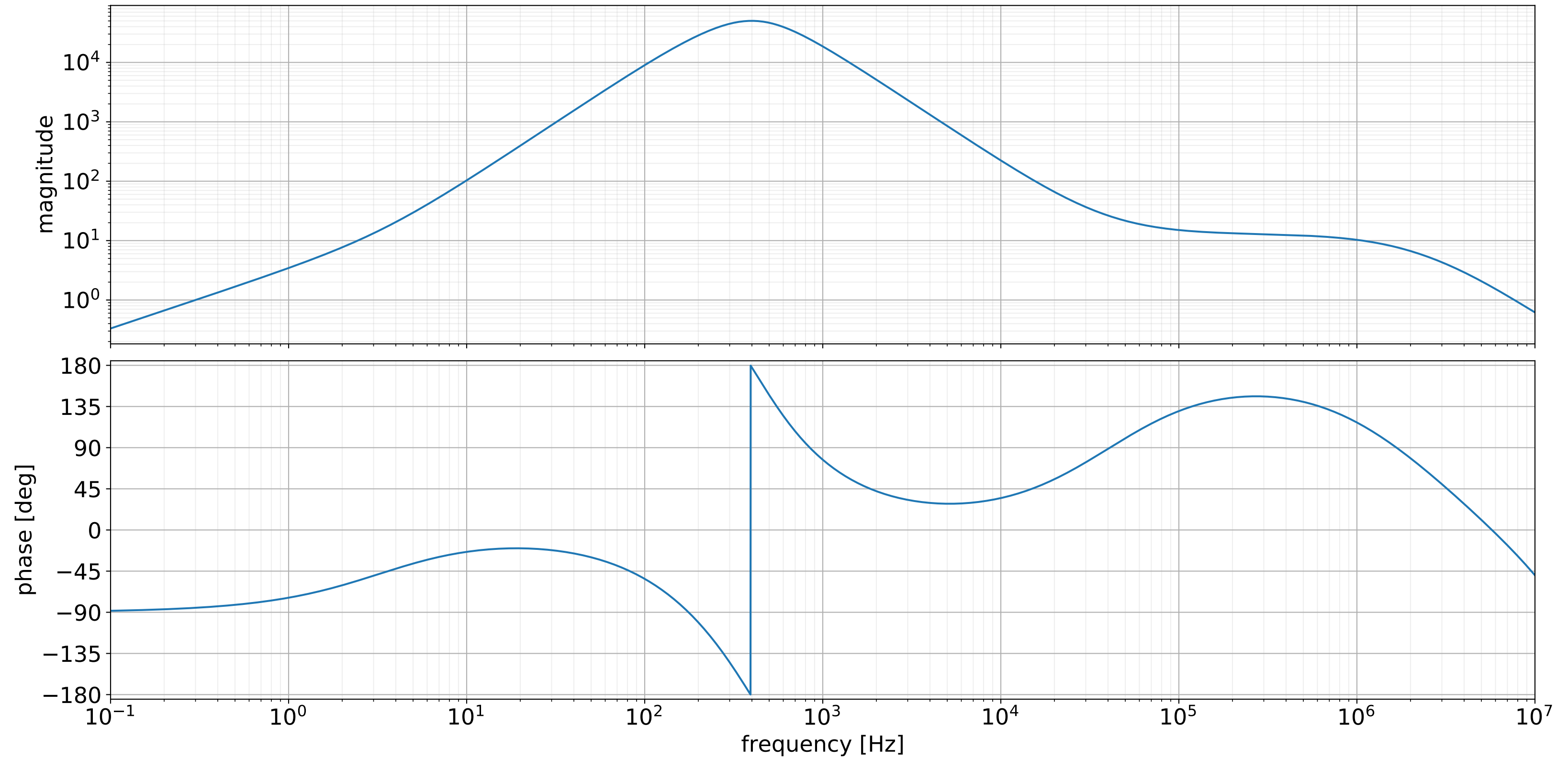
Transfer Function for the feedback circuit
