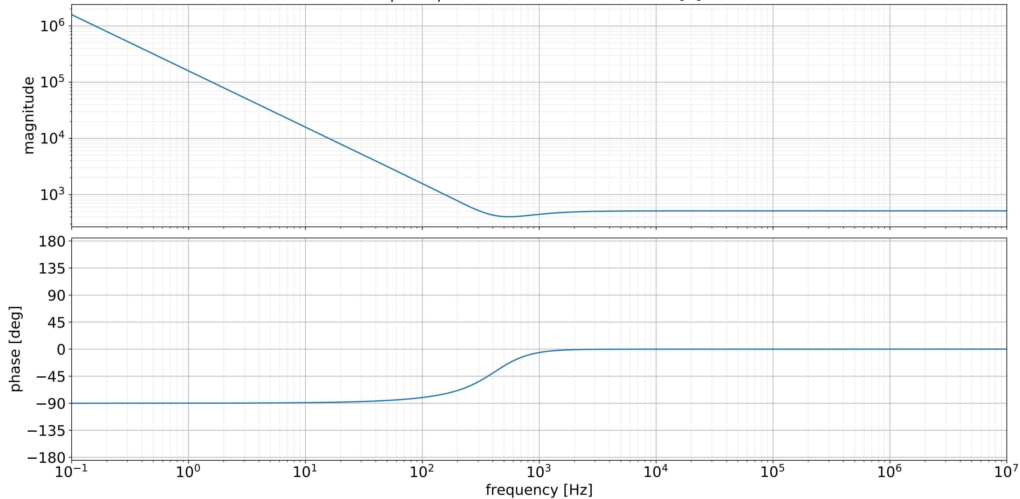
Input Impedance for the feedback Circuit [ \Omega ]
