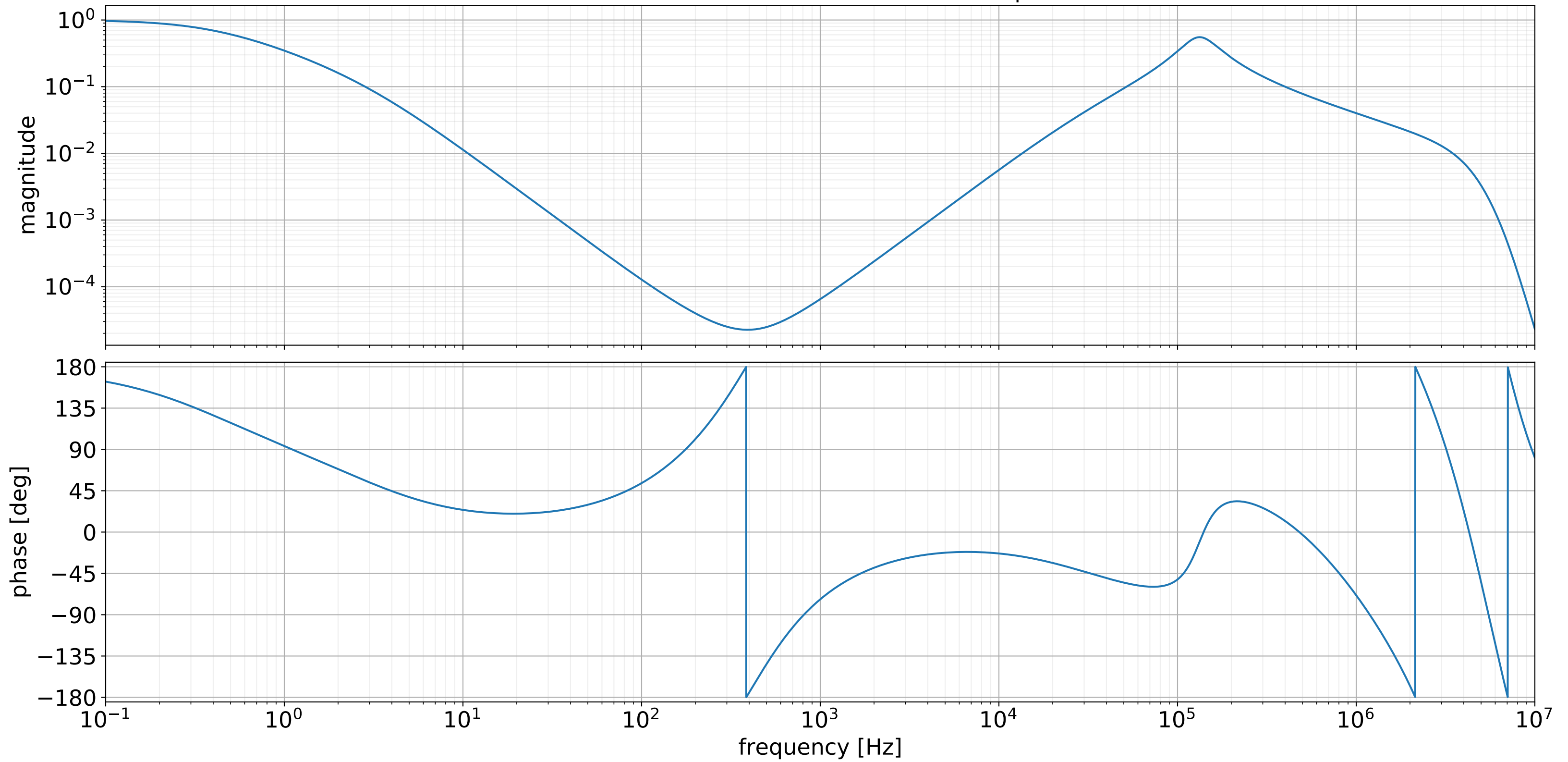
Transfer Function from PD to laser output
