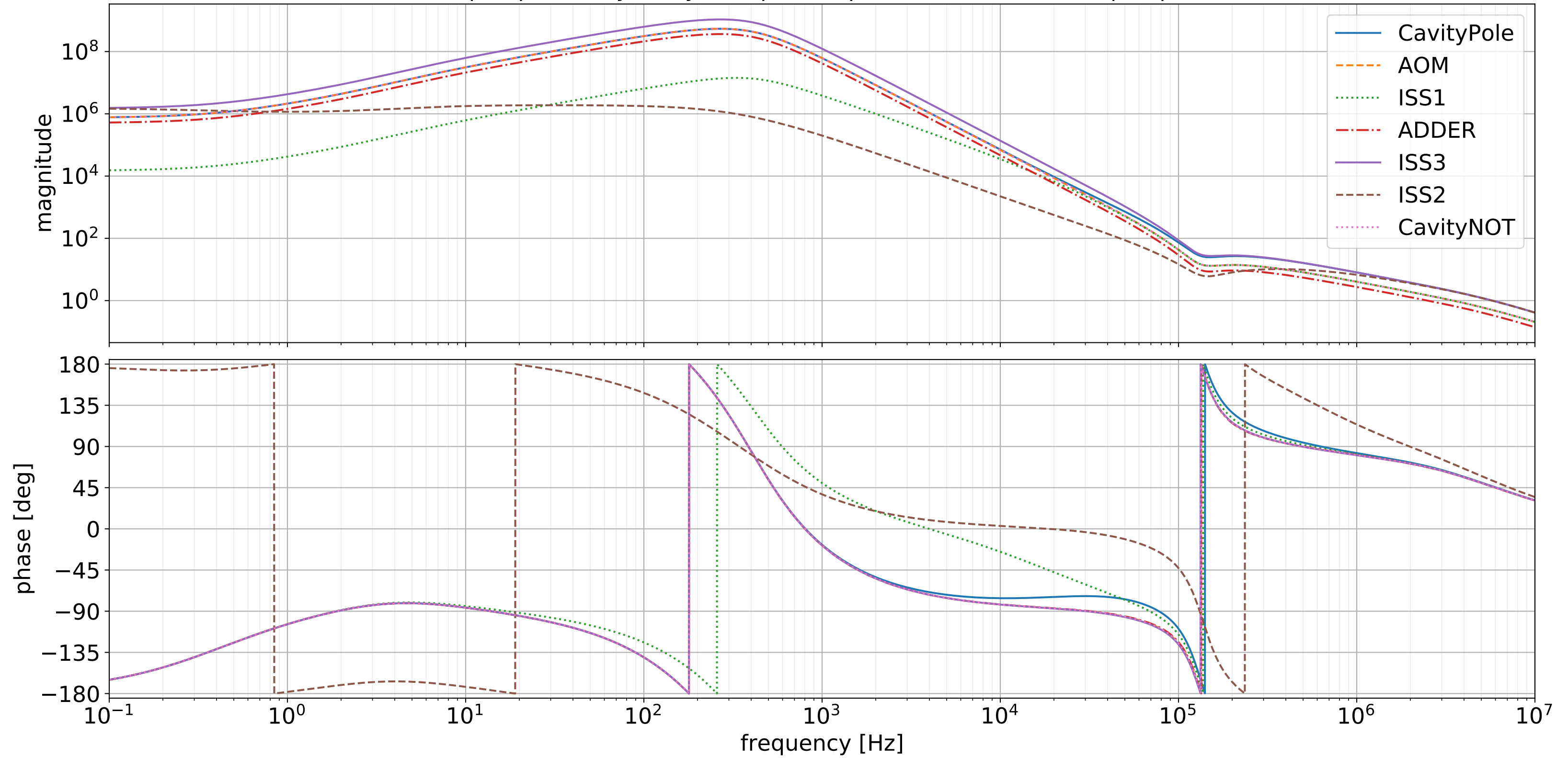
Opamp Stability Analysis (Open Loop Gain functions of all opamps)
