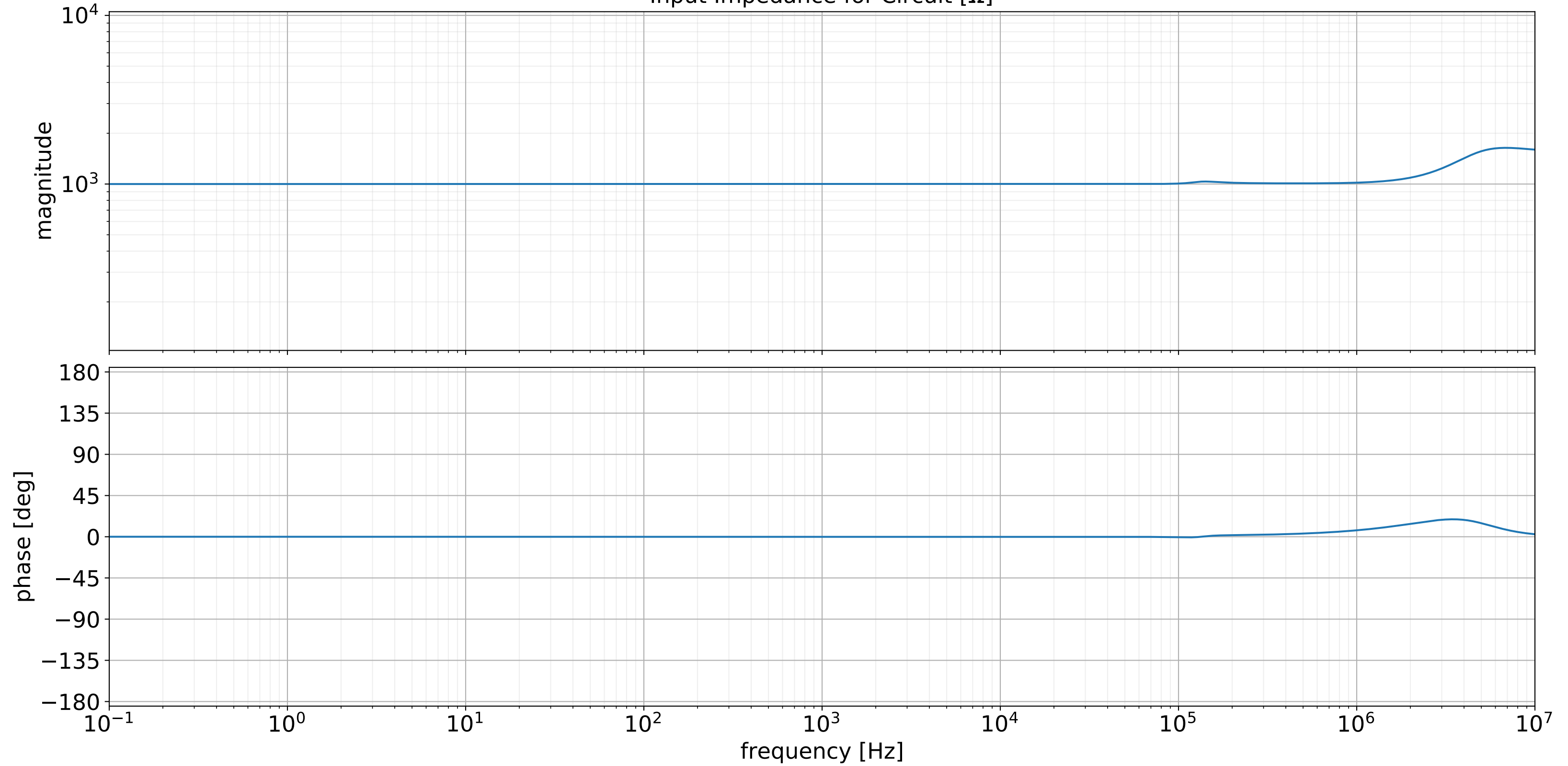
Input Impedance for Circuit [ \Omega ]
