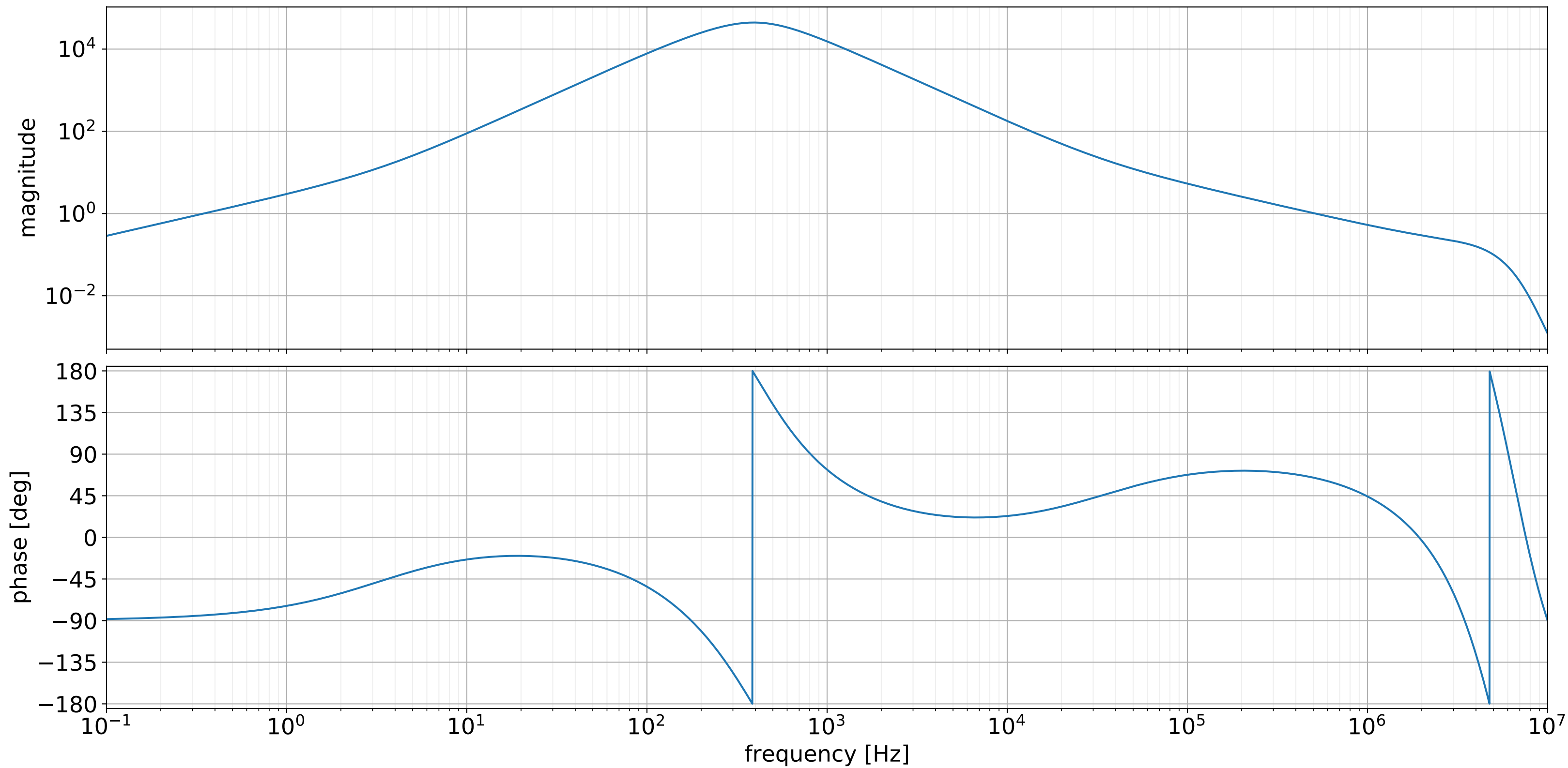
Transfer Function of feedback circuit
