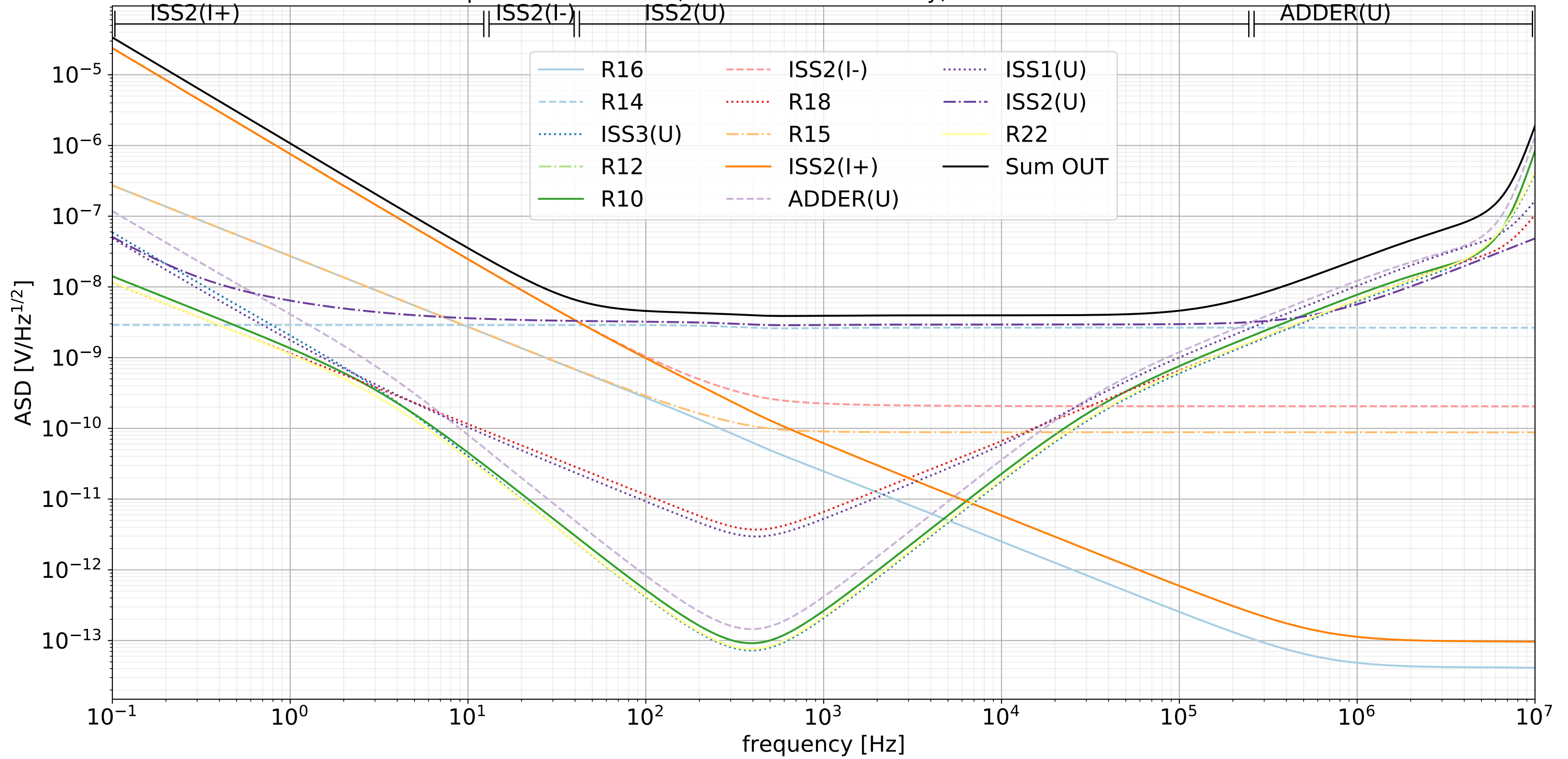
Input referred Noise (Dominant Sources only) in the feedback circuit
