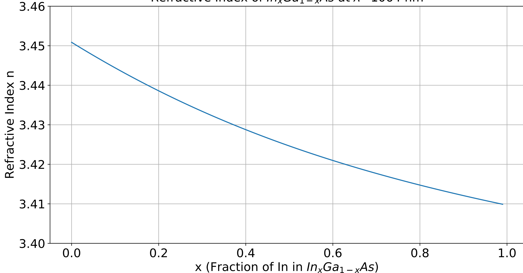
Refractive Index of In_xGa_{1-x}As at \lambda=1064 nm
