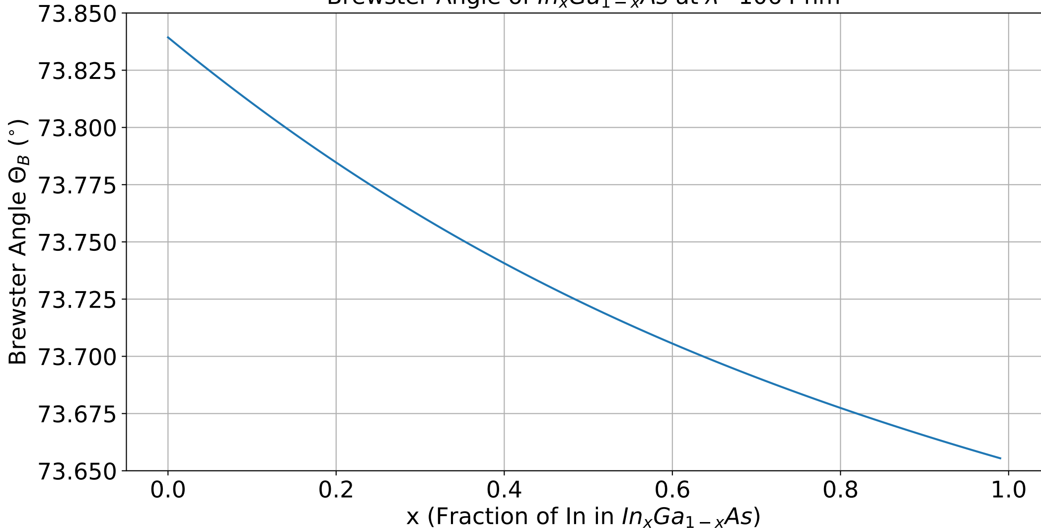
Brewster Angle of In_xGa_{1-x}As at \lambda=1064 nm
