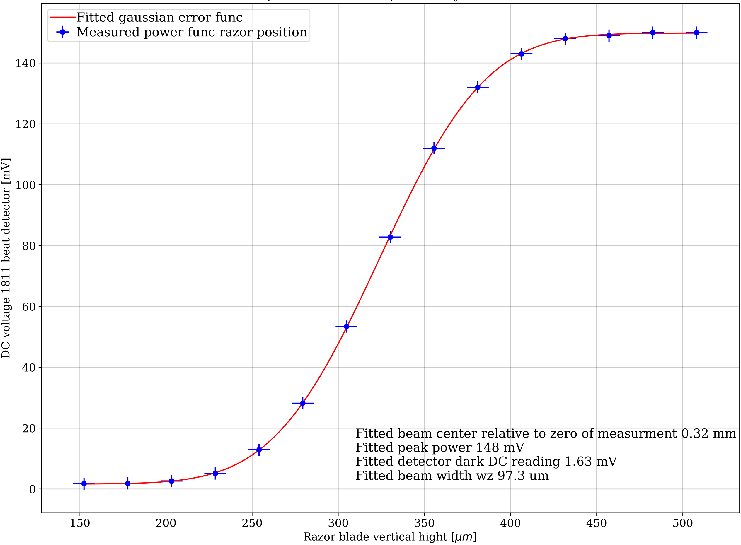
Razor blade profile of beam at post cavity BN detector with fit
