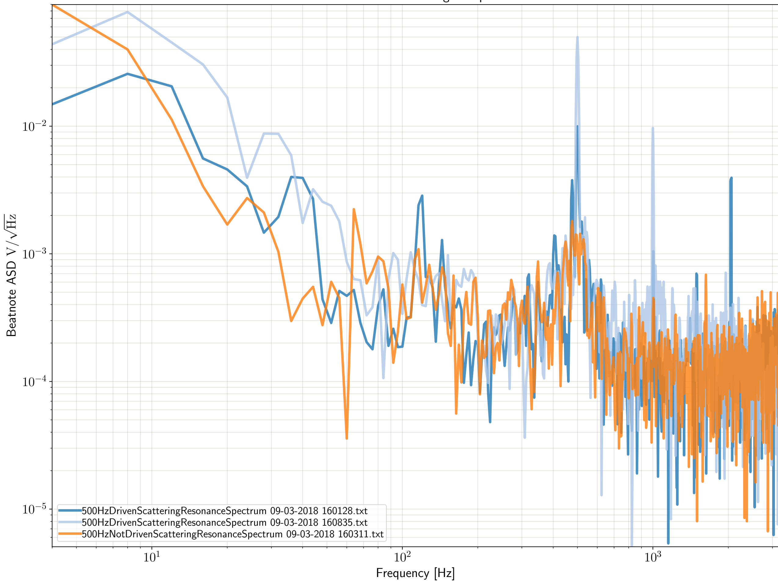
Driven vs Static 500 Hz Scattering Hump - Mar-09-2018
