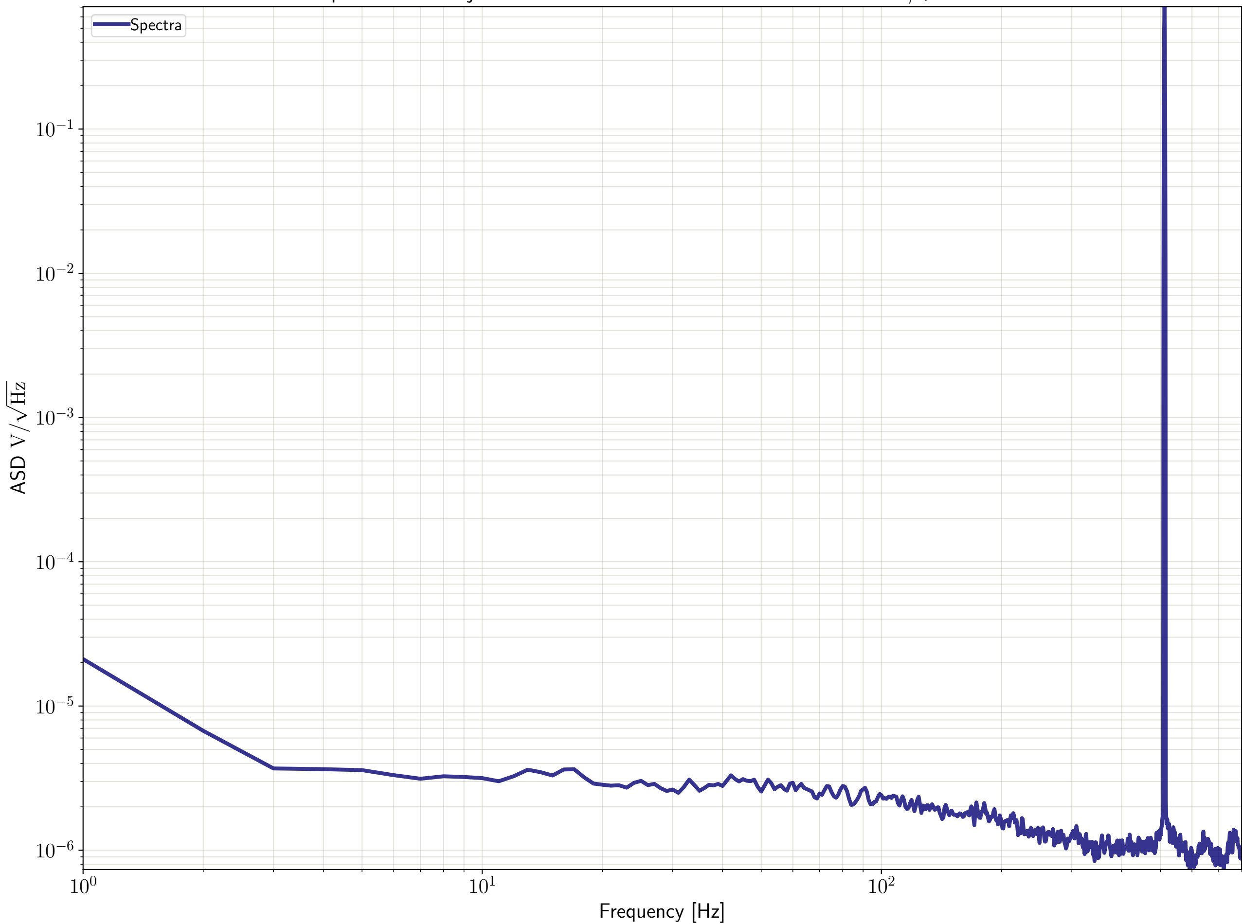
SR785 Response to Sine Injected at 512 Hz and 1 Vrms: Max ASD = 0.709 V/ \sqrt{\text{Hz}} - Feb-13-2018
