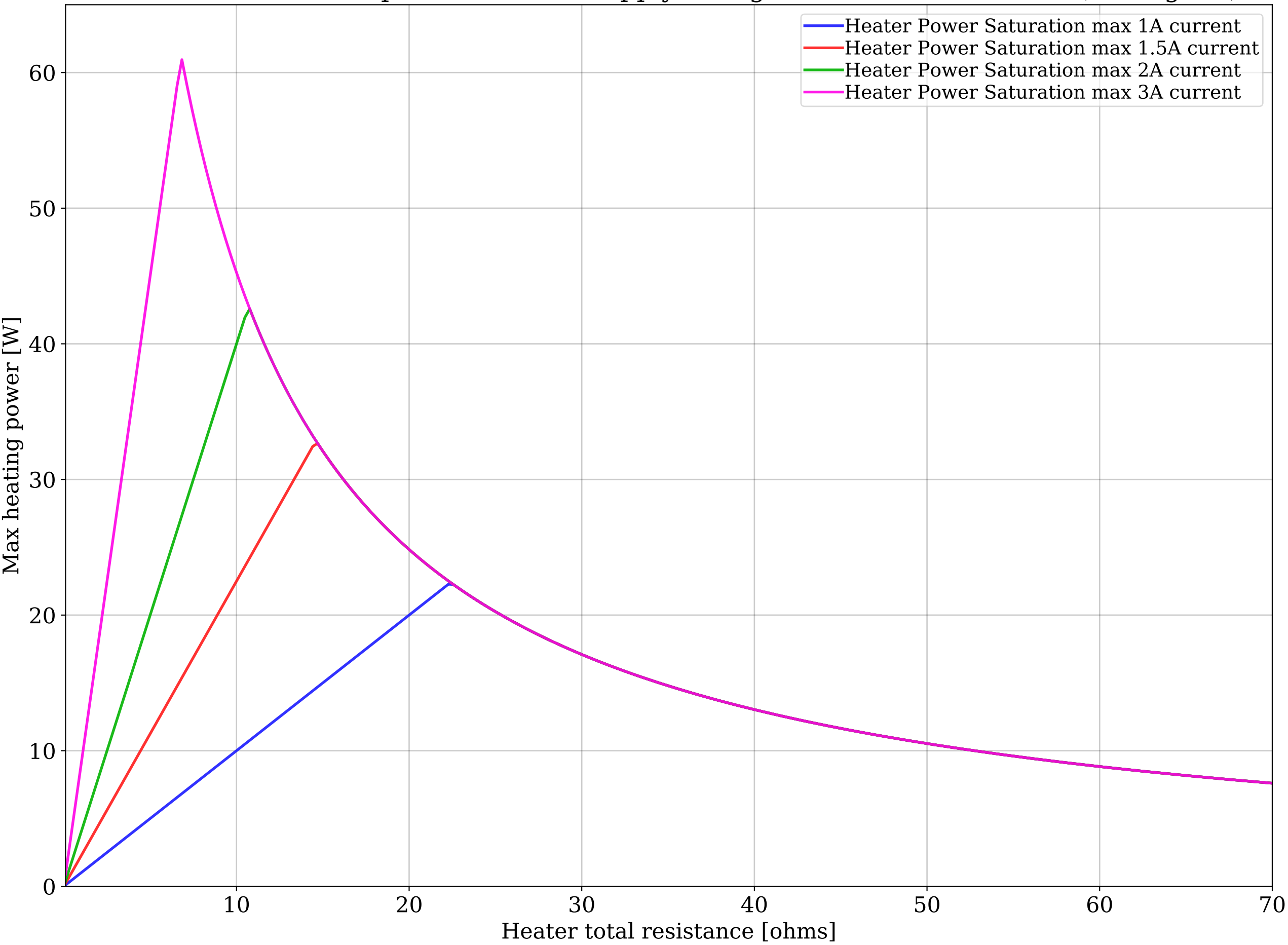
Maximum deliverable power for fixed supply voltage 24V and Max current (see legend)
