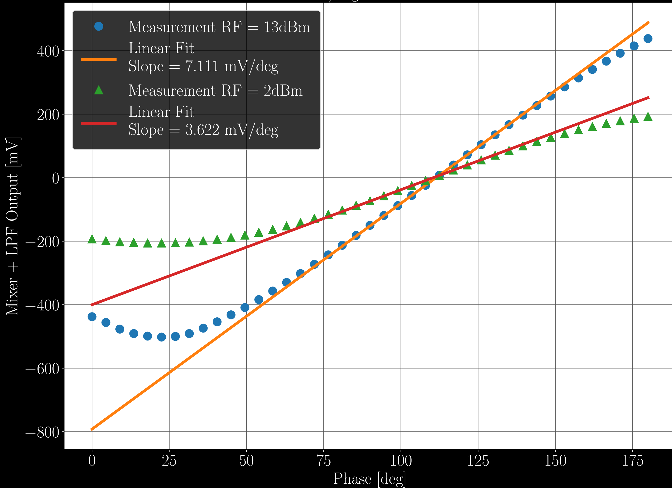
Mixer Calibration in mV/deg at 100 MHz with LO = 13 dBm
