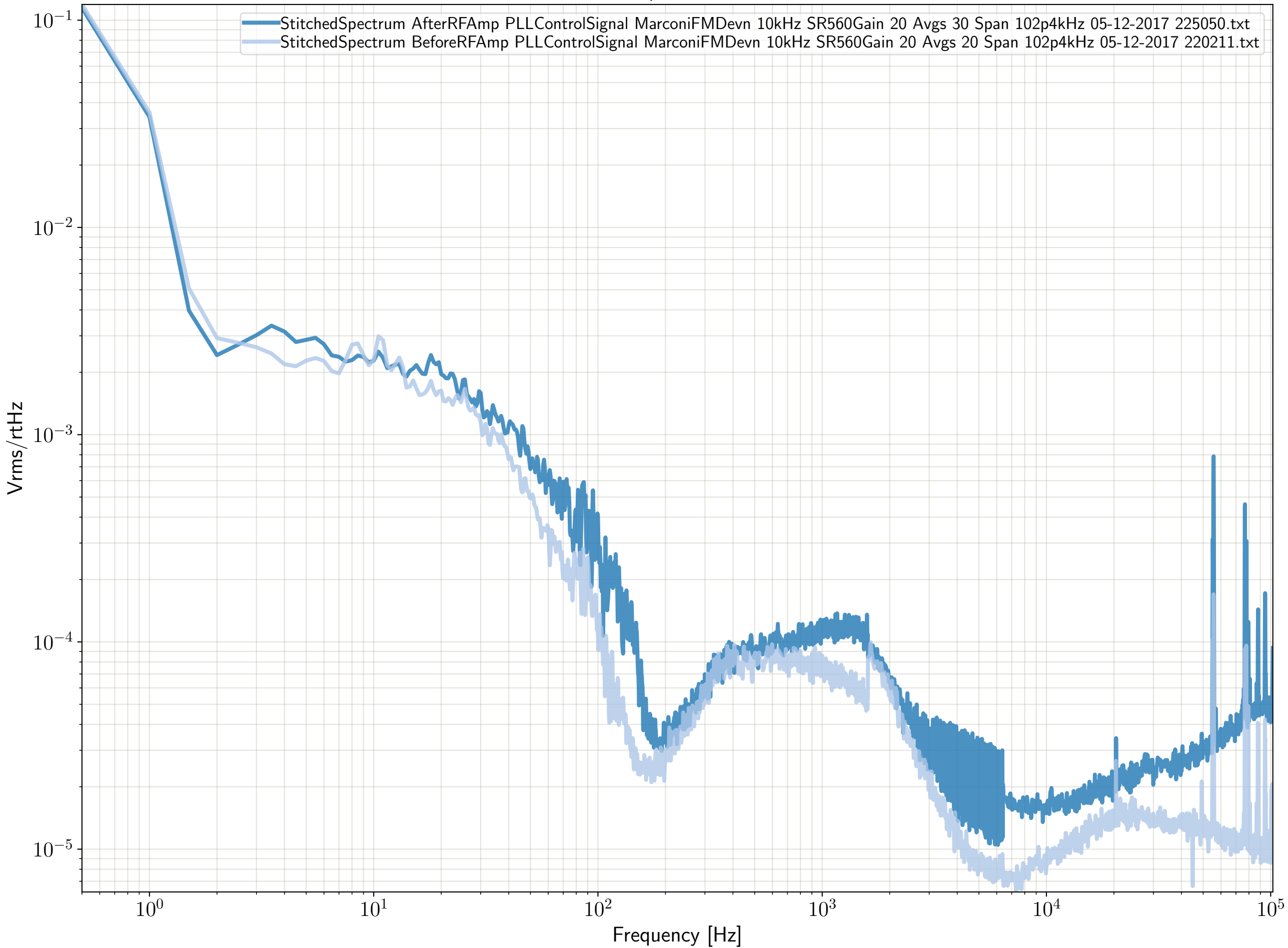
Before and After RF amp added to PLL - Dec-05-2017
