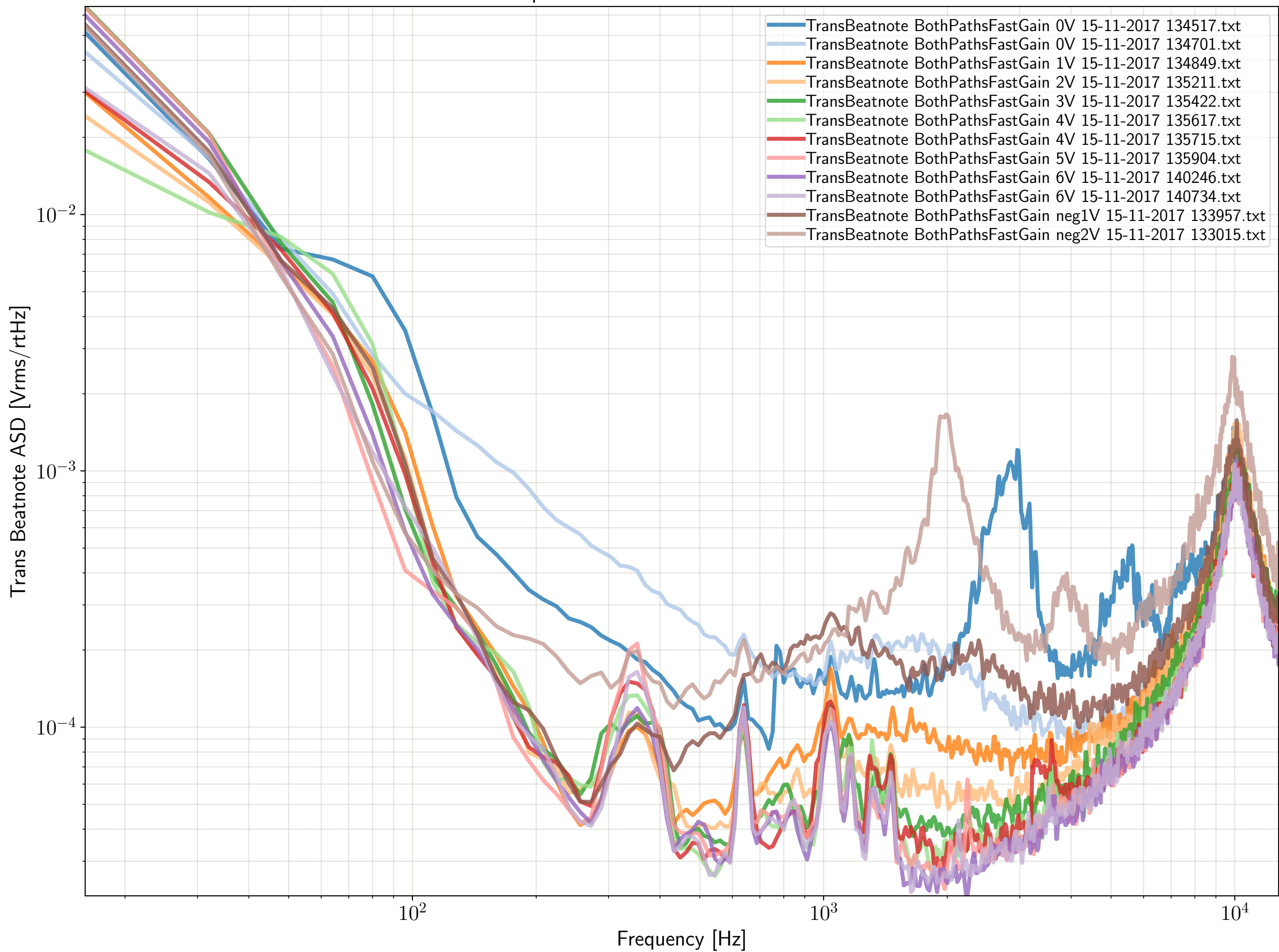
Trans Beatnote Spectra with different Fast Gain levels - Nov-15-2017
