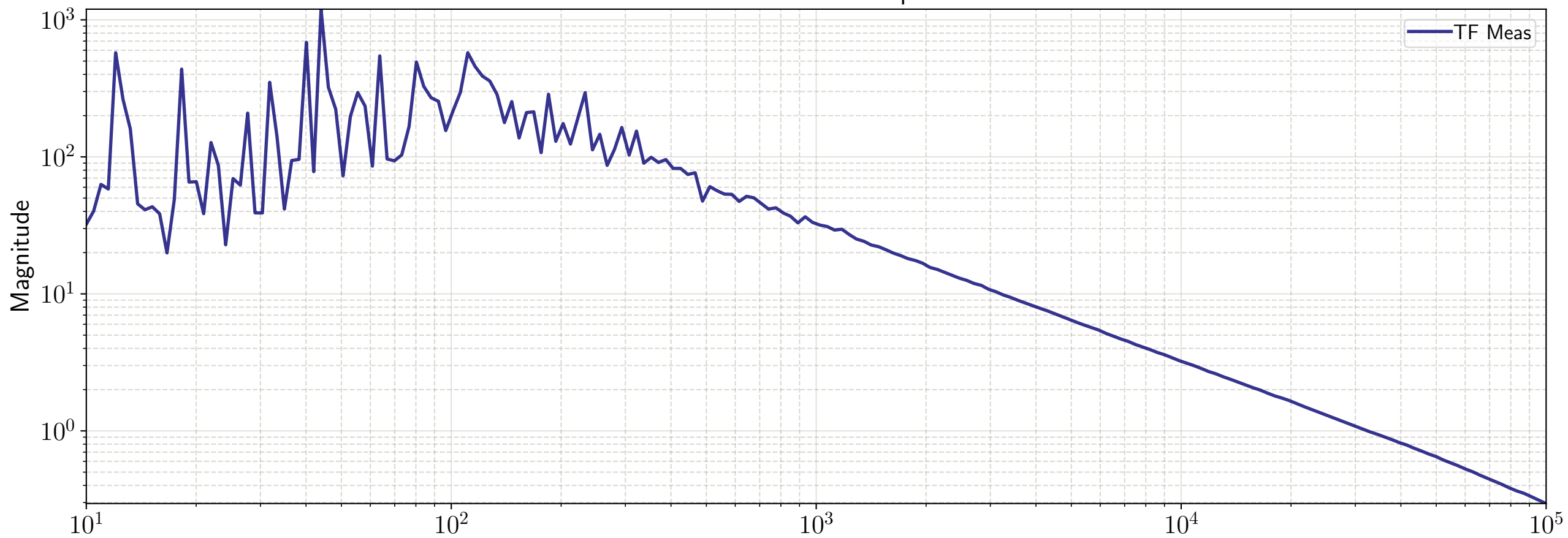
PLL OLG with FM Devn = 1 kHz and Preamp Gain = 2000 - Nov-12-2017
