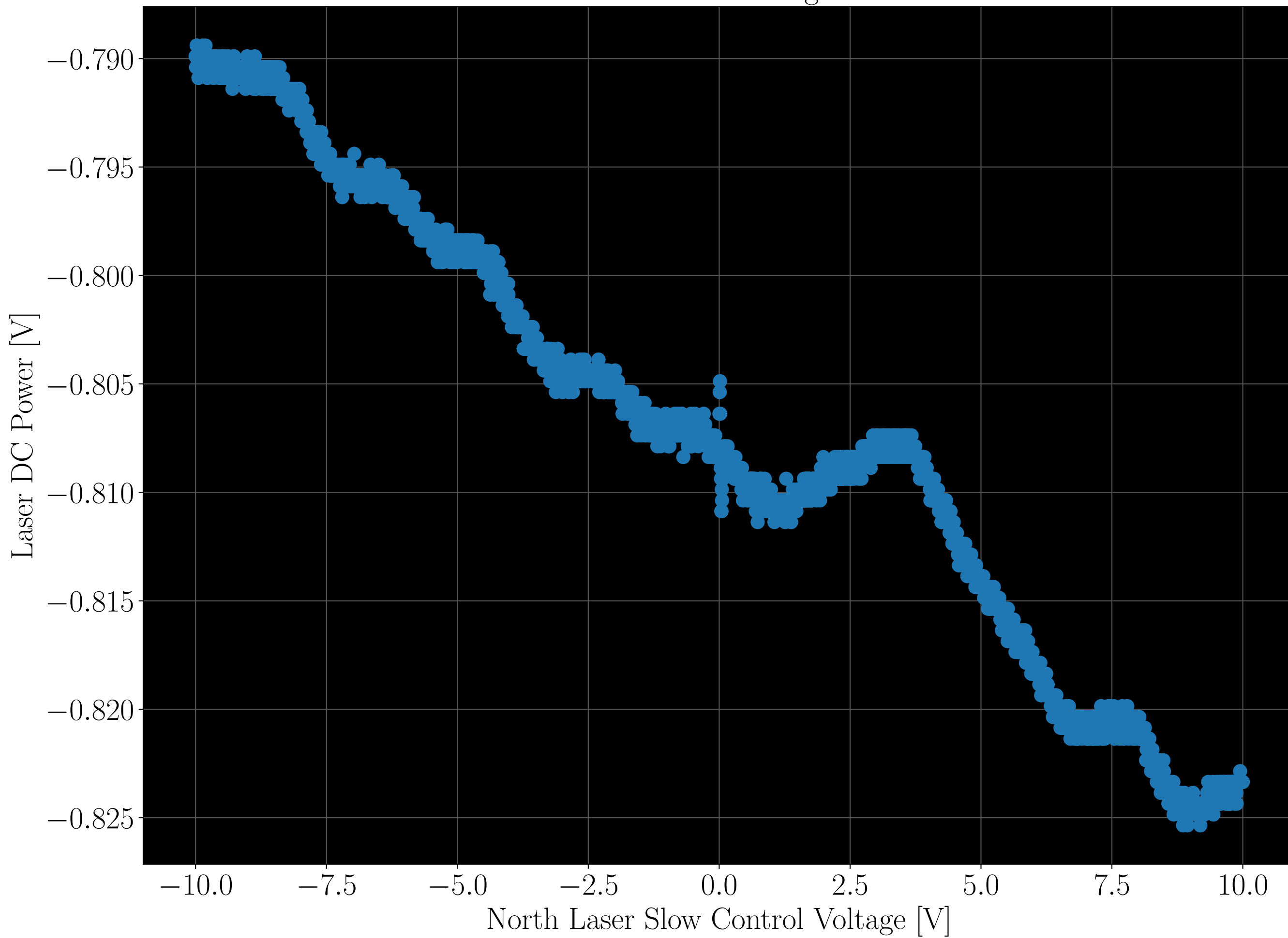
North Laser Slow Control Voltage vs Laser Power
