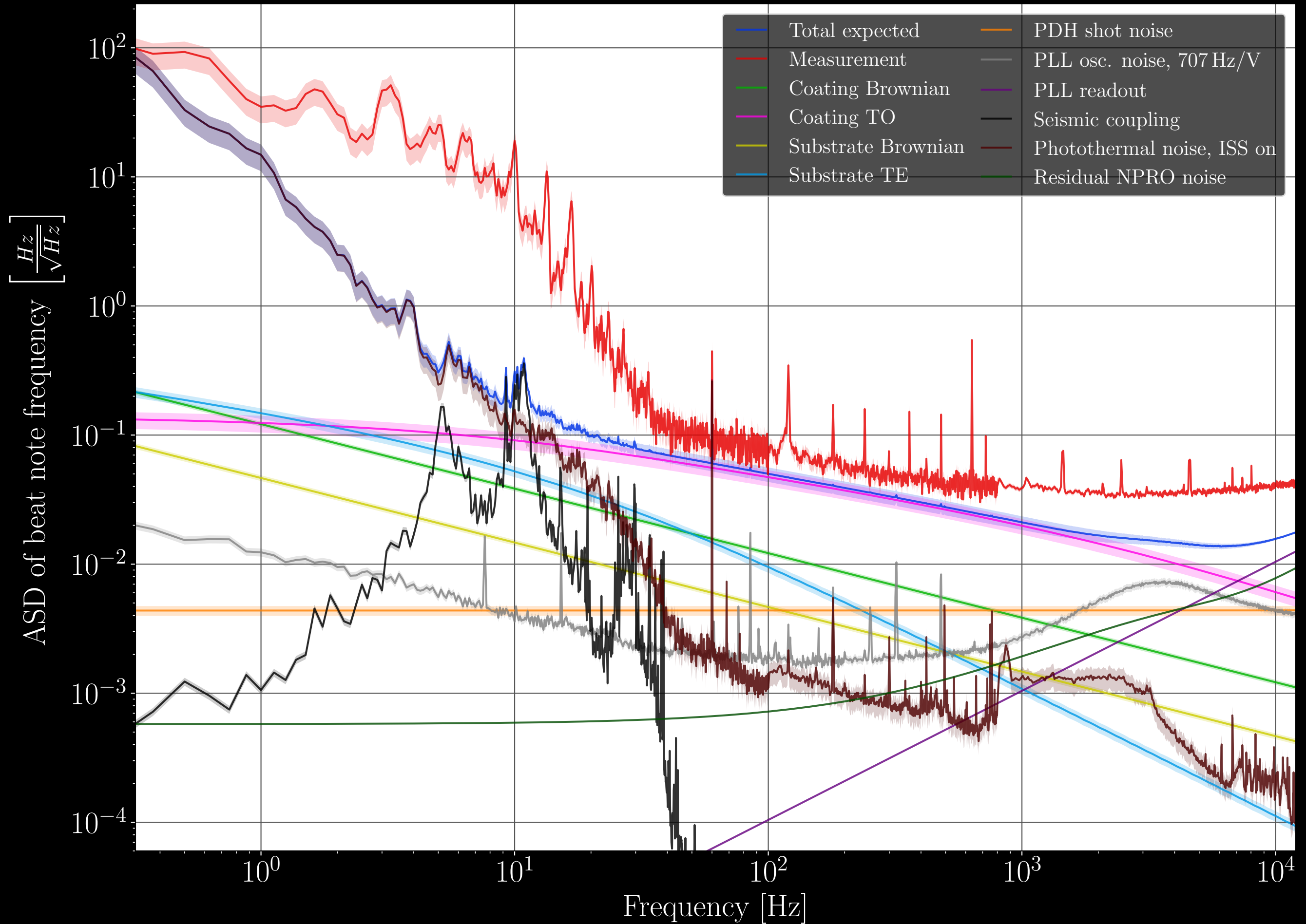
Noise budget for two 3.68-cm cavities with GaAs/Al 0.92 Ga 0.08 As Bragg mirrors
