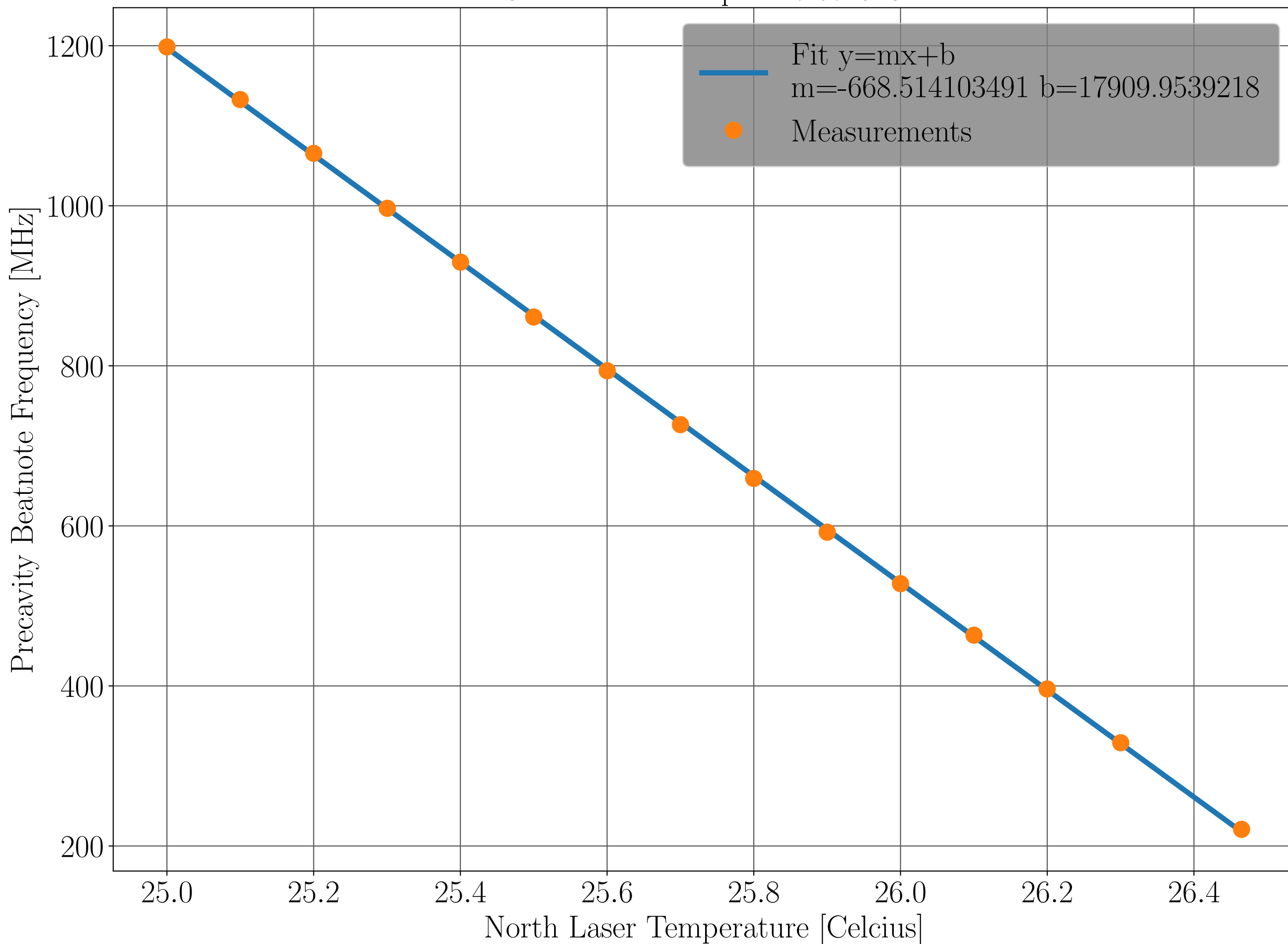
North Laser Temp Vs Precavity Beatnote Frequency South Laser Temp = 47.0749 C
