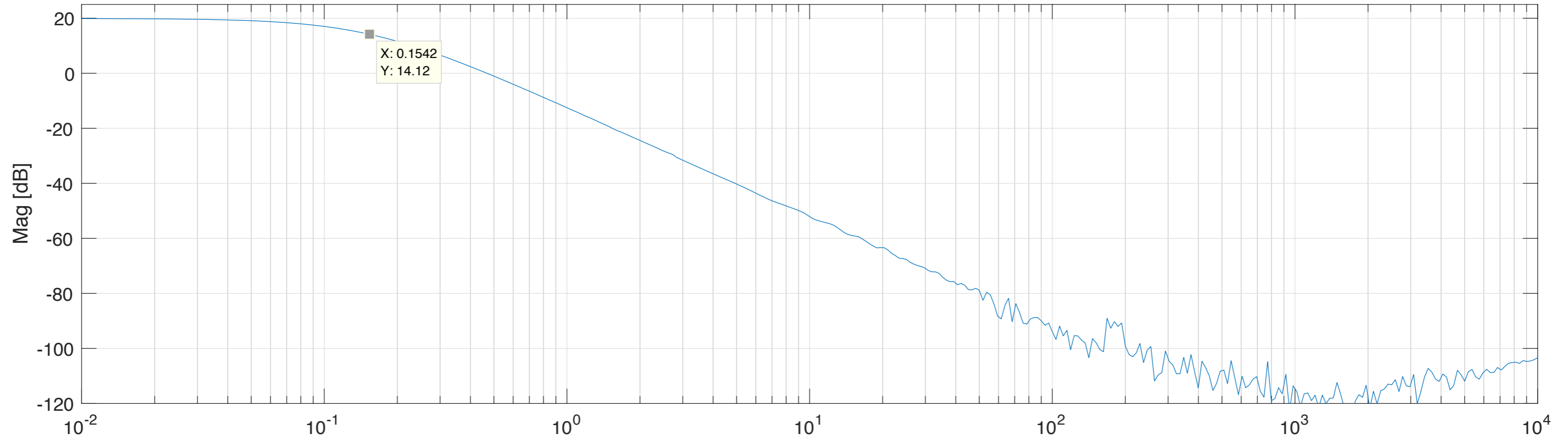
2016-10-17 TF Sallen Key 2nd-order LP filter
