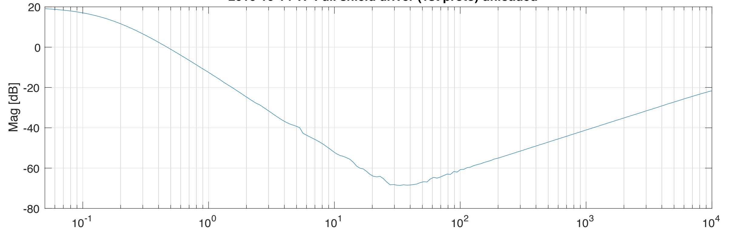
2016-10-14 TF Full shield driver (1st proto) unloaded
