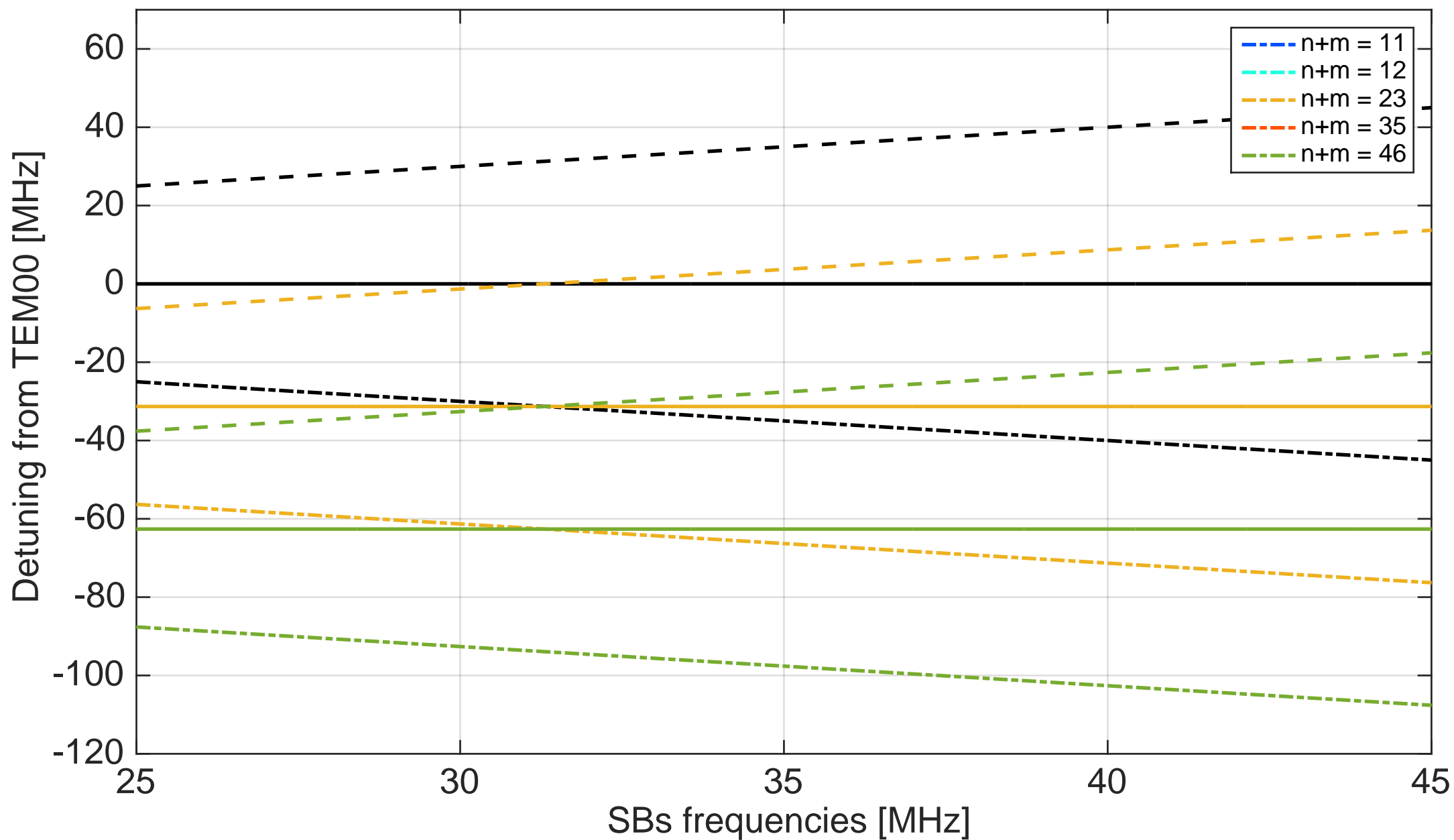
HOM for a cavity with L=3.68\text{cm} and R1=R2=1\text{m}
