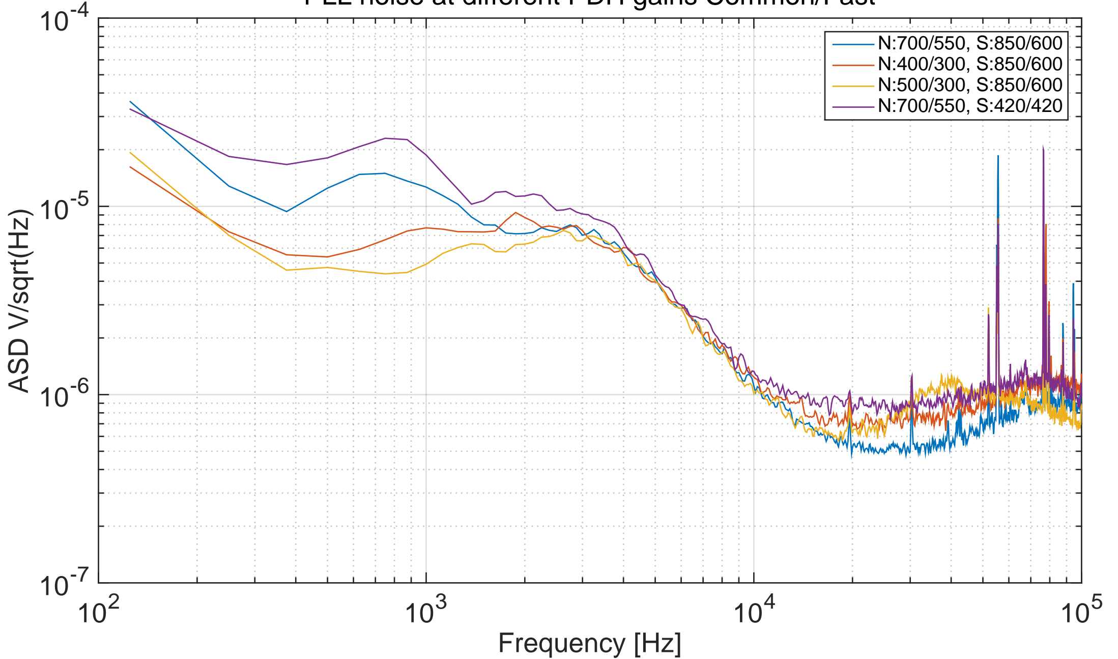
PLL noise at different PDH gains Common/Fast
