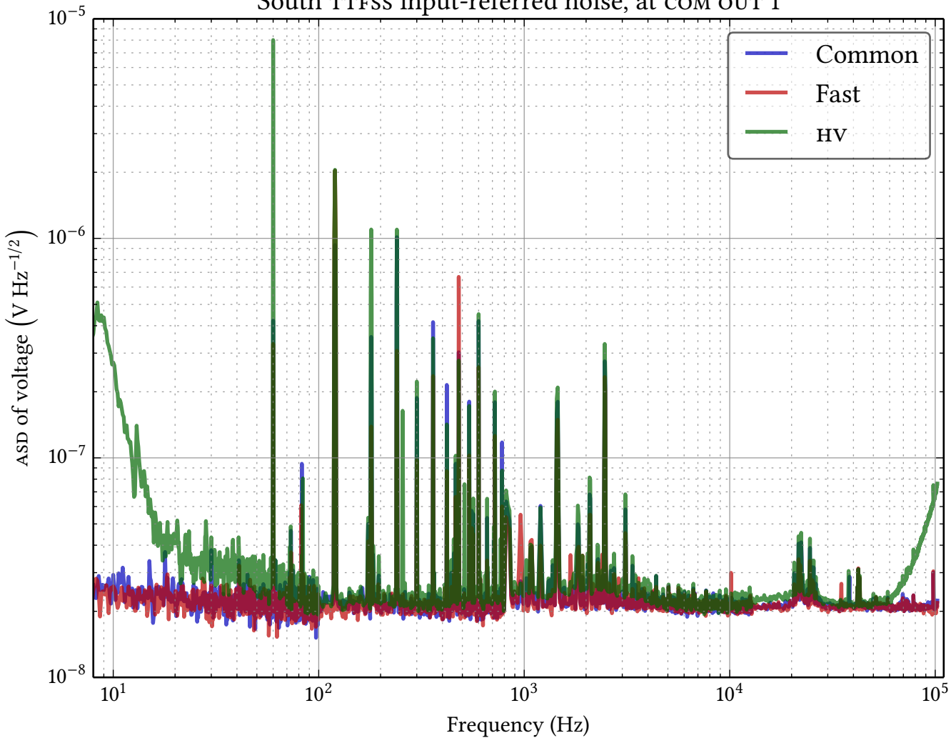
South TTFSS input-referred noise, at COM OUT 1
