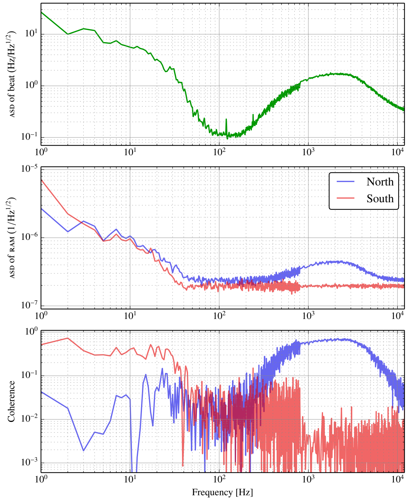
RAM coherence measurements for AlGaAs cavities
