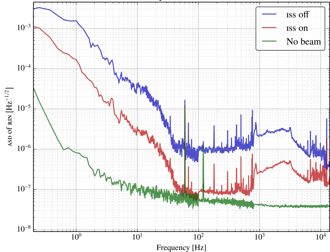
RIN of south cavity transmission, 2014-09-11
