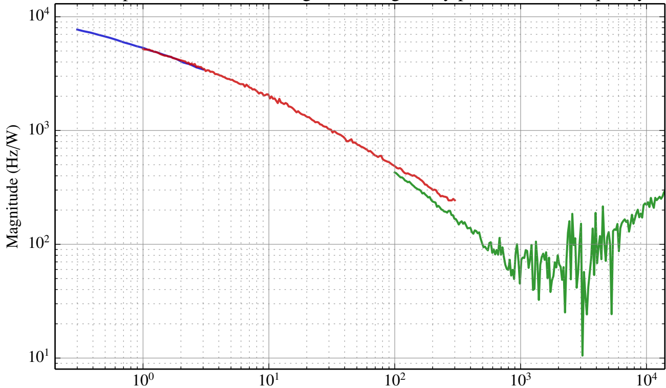
South photothermal TF, taking circulating cavity power to beat frequency
