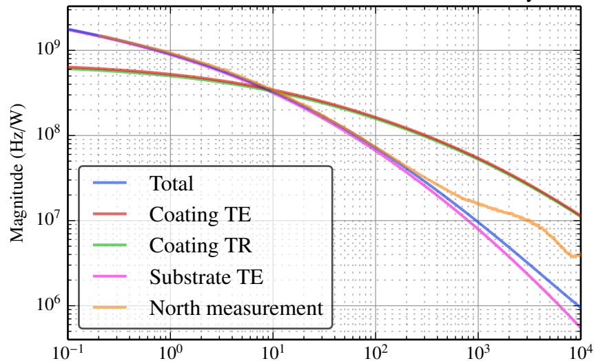
Photothermal TF for a two-mirror AlGaAs cavity
