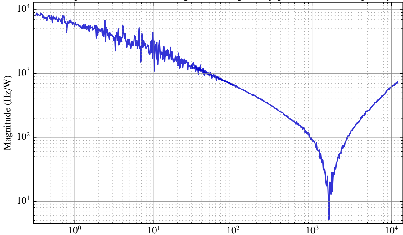
North photothermal TF, taking circulating cavity power to beat frequency
