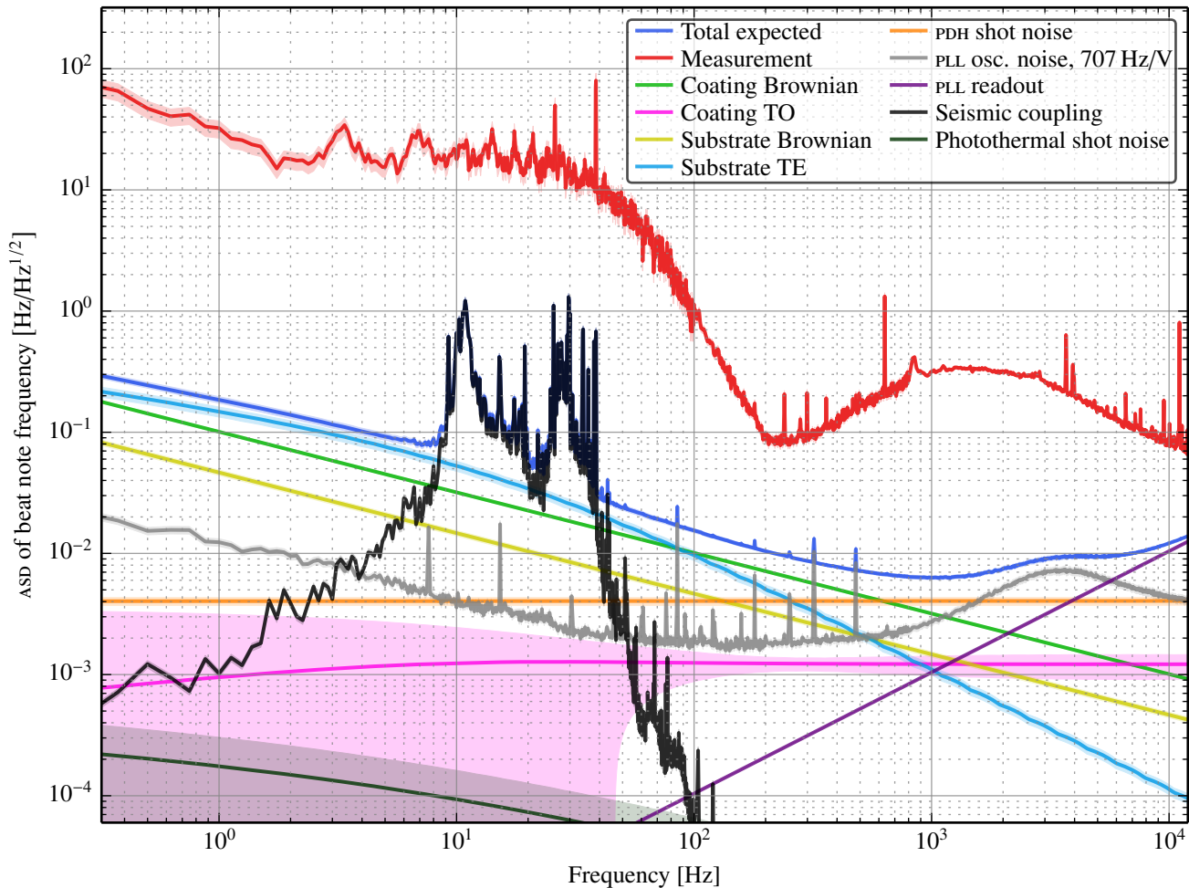
Noise budget for two 3.68-cm cavities with GaAs/Al 0.92 Ga 0.08 As Bragg mirrors
