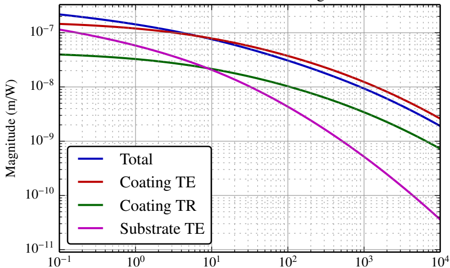
Photothermal transfer function for a single AlGaAs mirror
