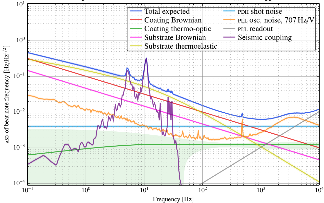
Noise budget for two 3.68-cm cavities with GaAs/Al 0.92 Ga 0.08 As Bragg mirrors
