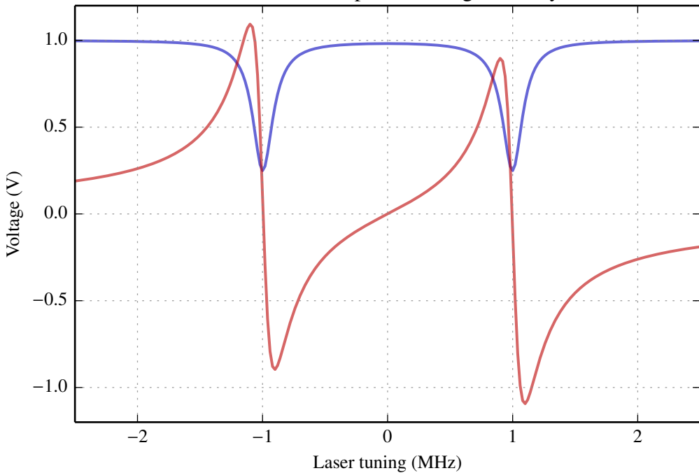
Simulated sweep of birefringent cavity
