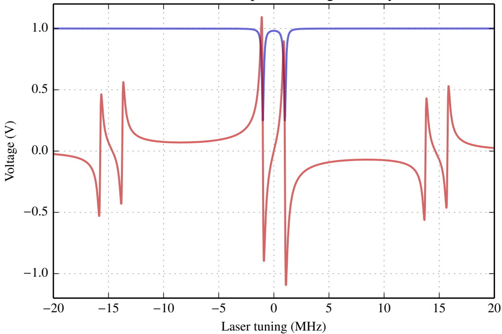
Simulated sweep of birefringent cavity
