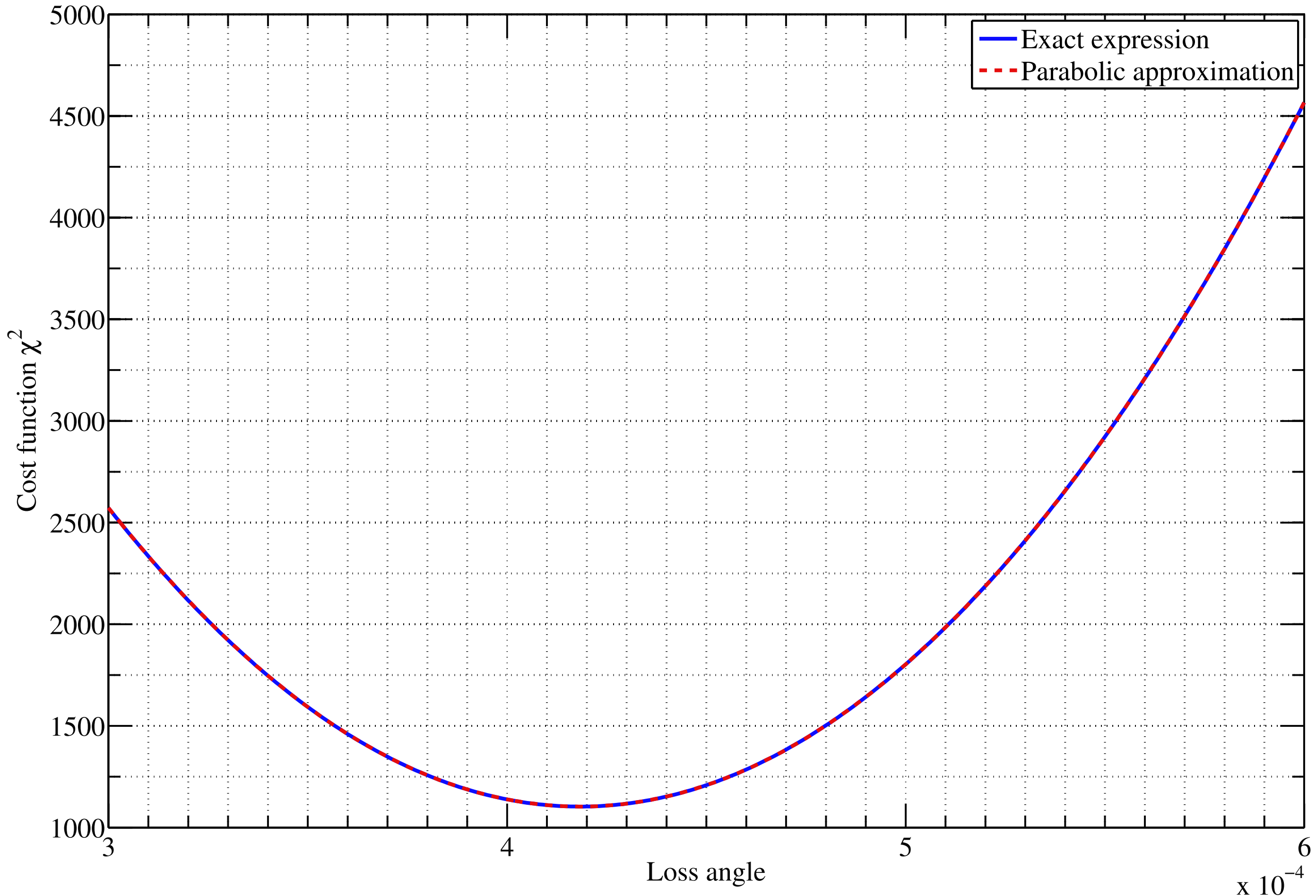
Cost function for a fit from 26 Hz to 405 Hz.
