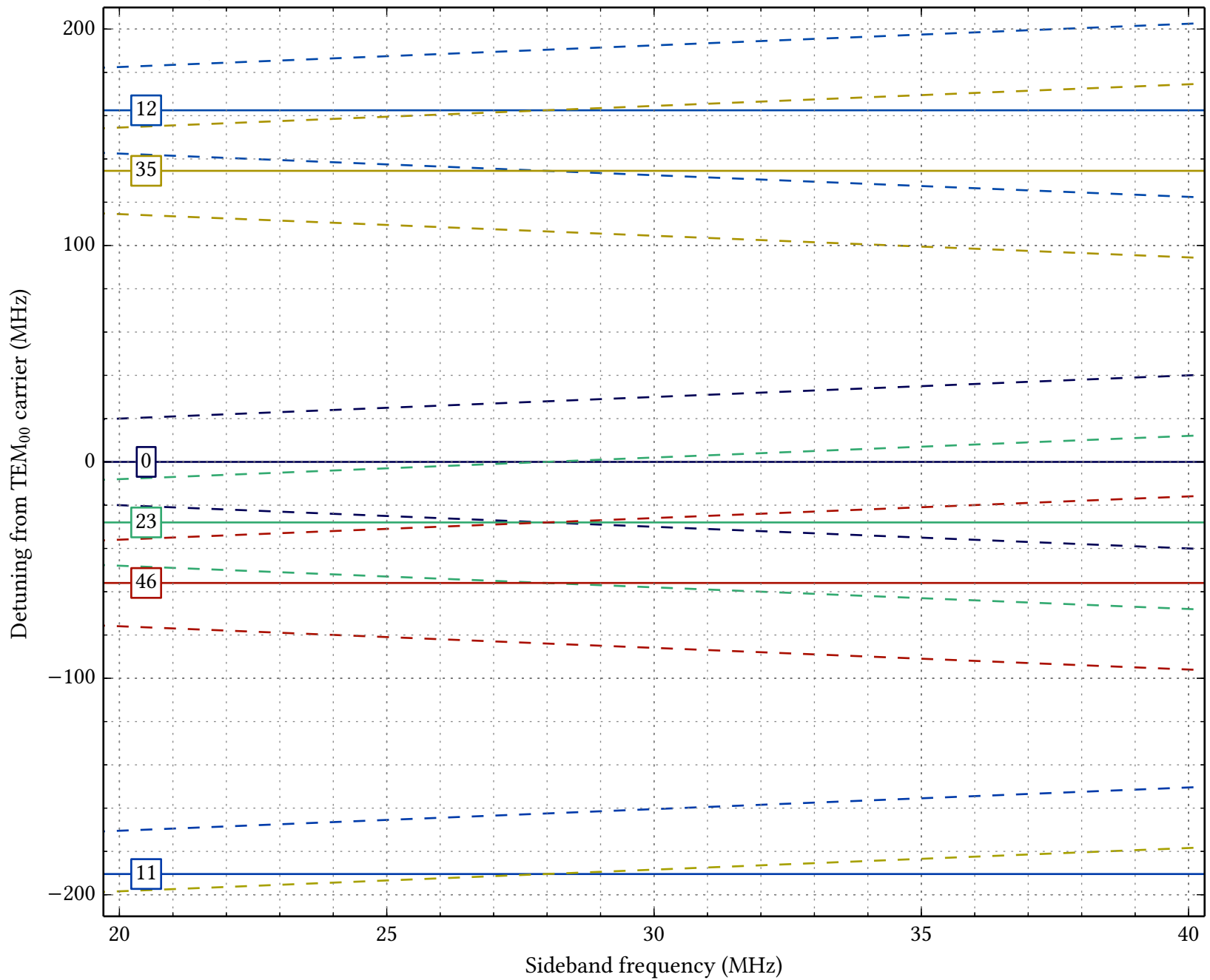
Higher-order modes for a Fabry-Pérot cavity with L = 3.7 cm and R_1 = R_2 = 1.0 m
