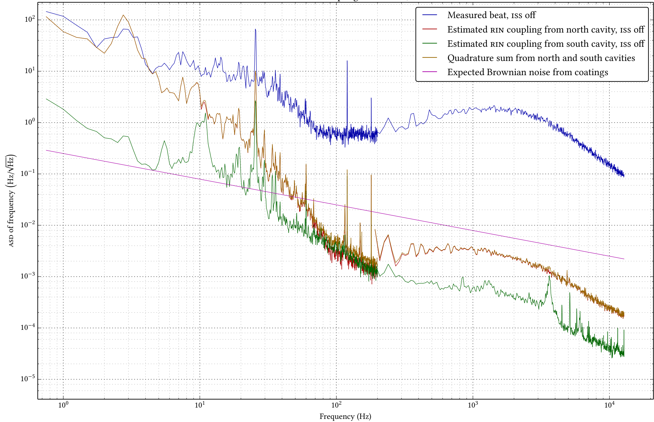
Estimated RIN-to-beat coupling with iss off; 2013-10-25
