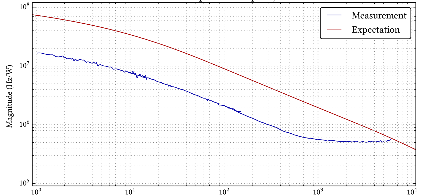
Transfer function from incident power to frequency fluctuation, 2013-10-17
