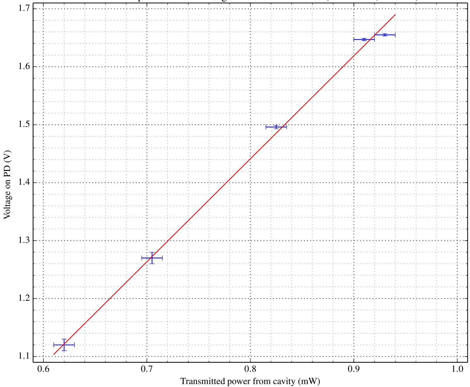
Transmitted power versus voltage on transmission PD (PDA10CS, +30 dB)
