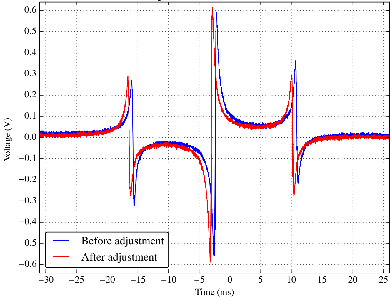
South PDH error signal (TTFSS common OUT1), 2013-09-23
