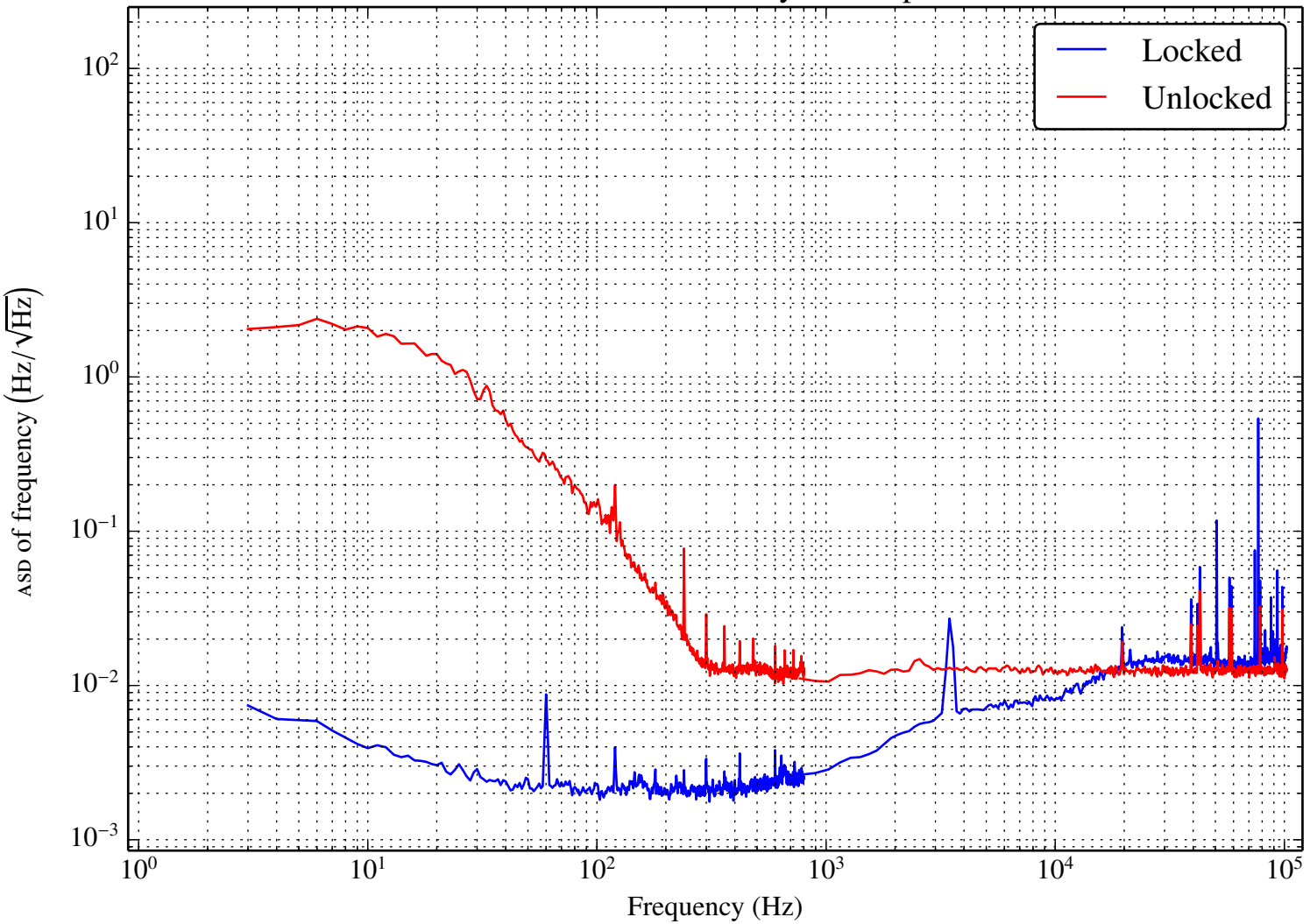
Noise of south cavity PDH loop
