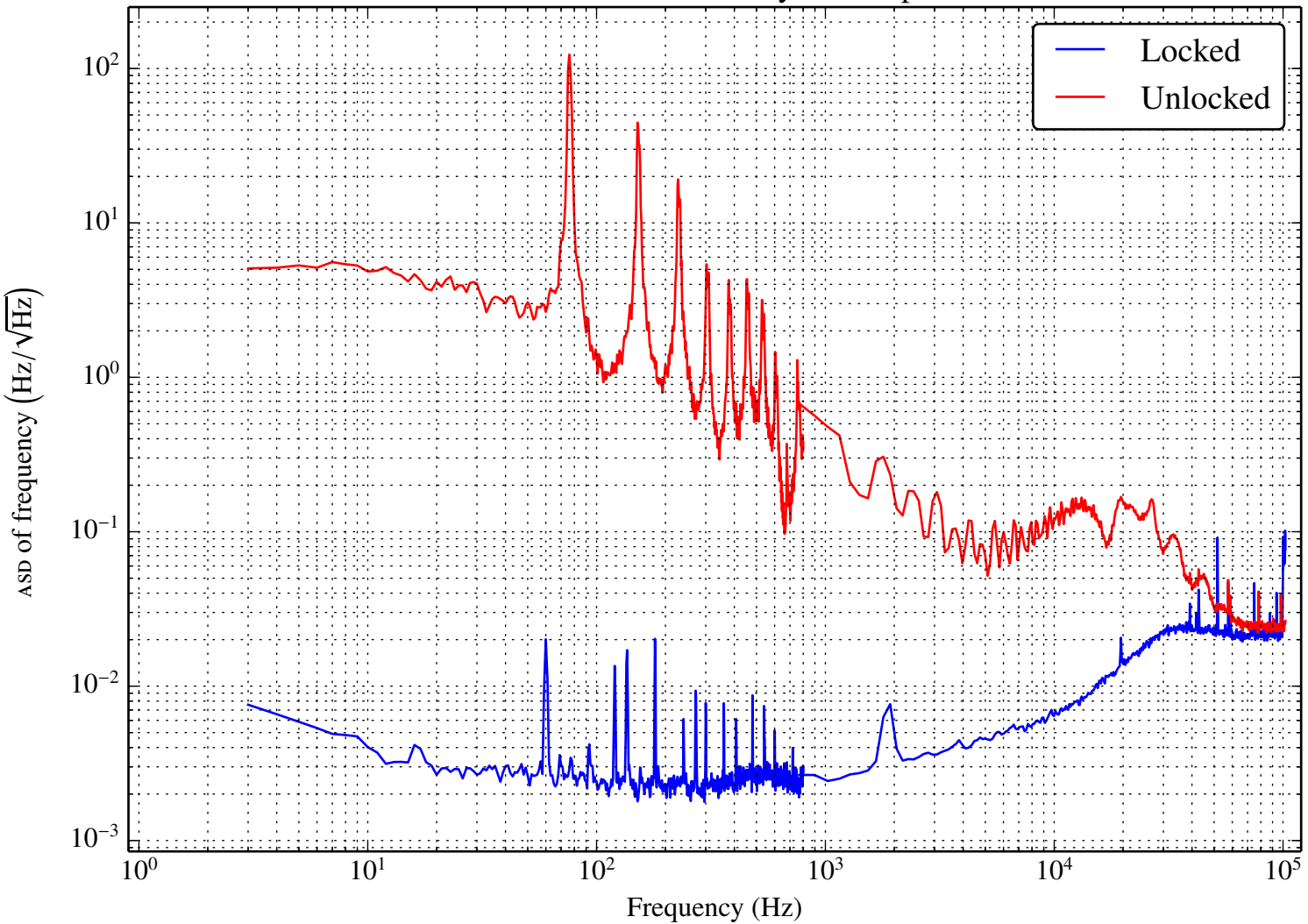
Noise of north cavity PDH loop
