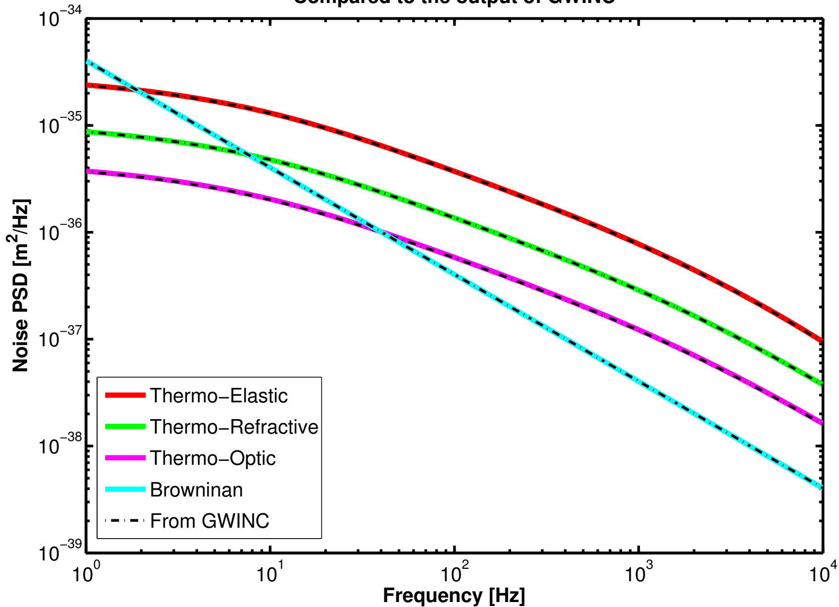
Coating noises calculated by the 'CoatingThermalNoiseCalc' code Compared to the output of GWINC
