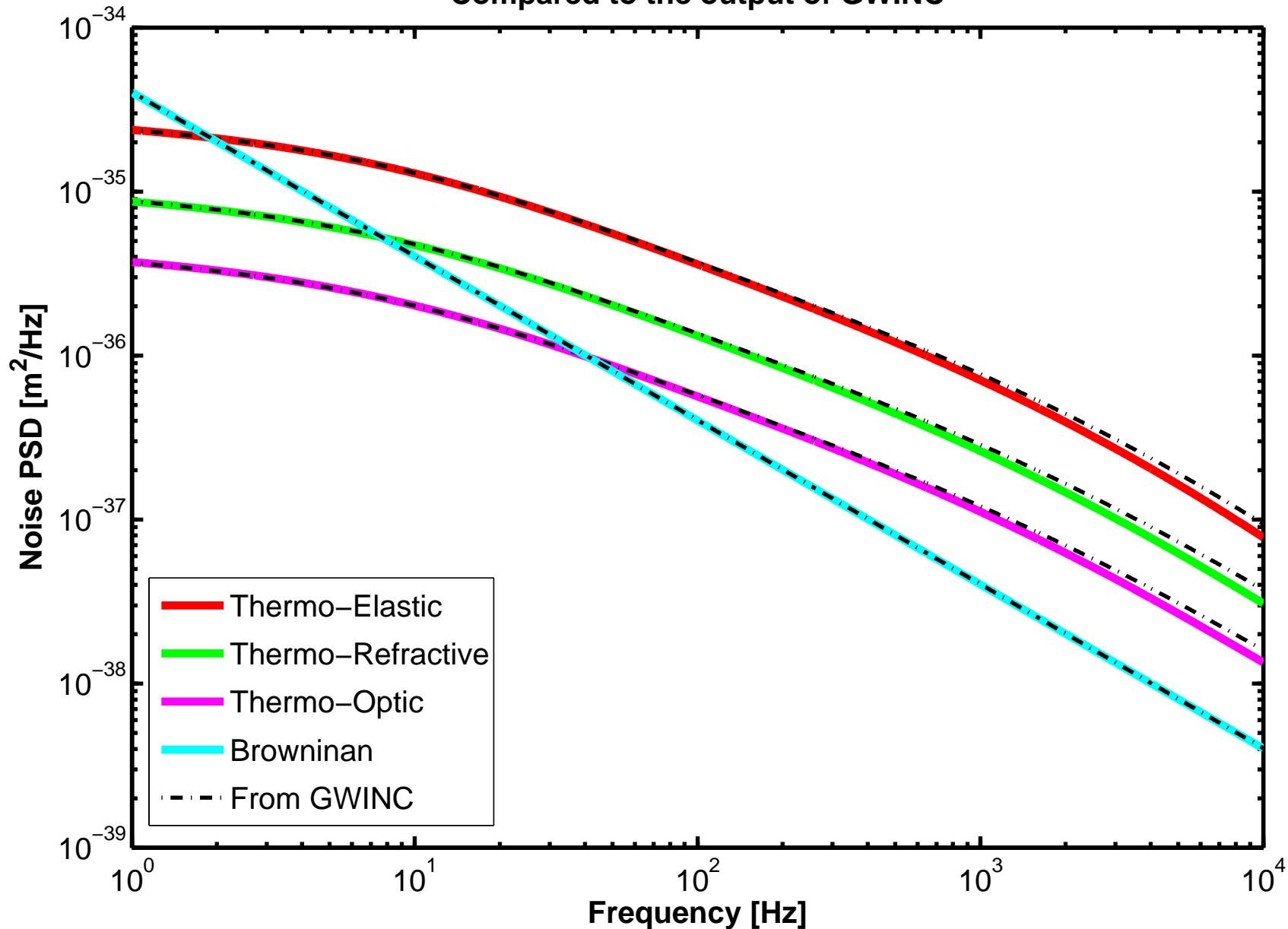
Coating noises calculated by the 'CoatingThermalNoiseCalc' code Compared to the output of GWINC
