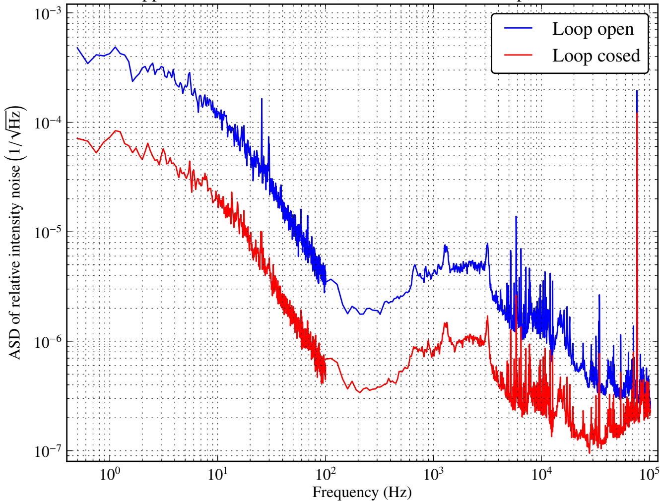
RIN suppression with a G = 500 , 30-kHz bandwidth loop; 2013-09-04
