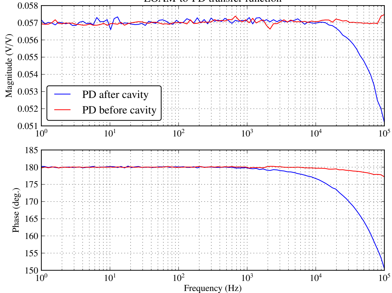
EOAM-to-PD transfer function
