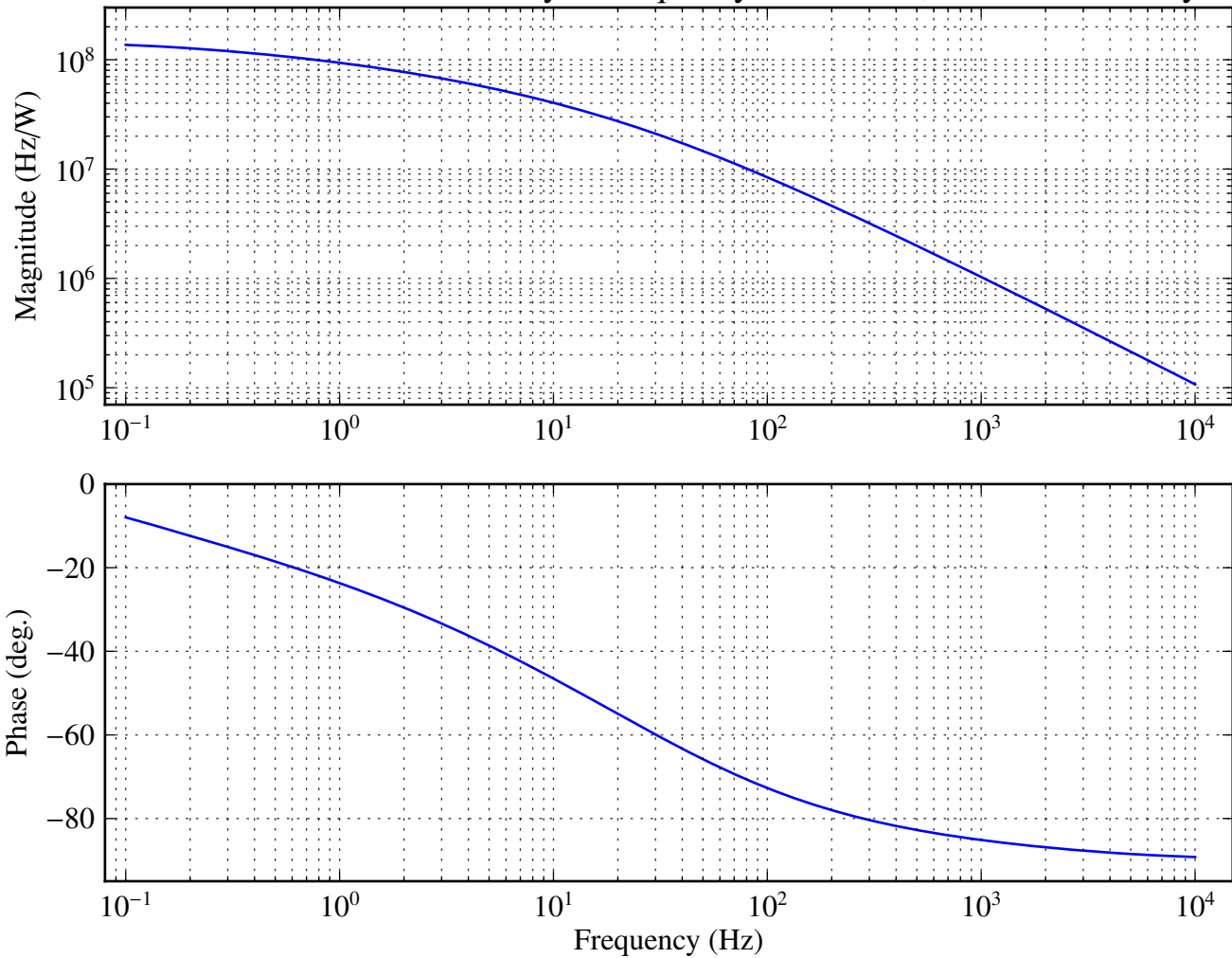
Transfer function of intensity to frequency for a 1.45'', F = 10\,000 cavity
