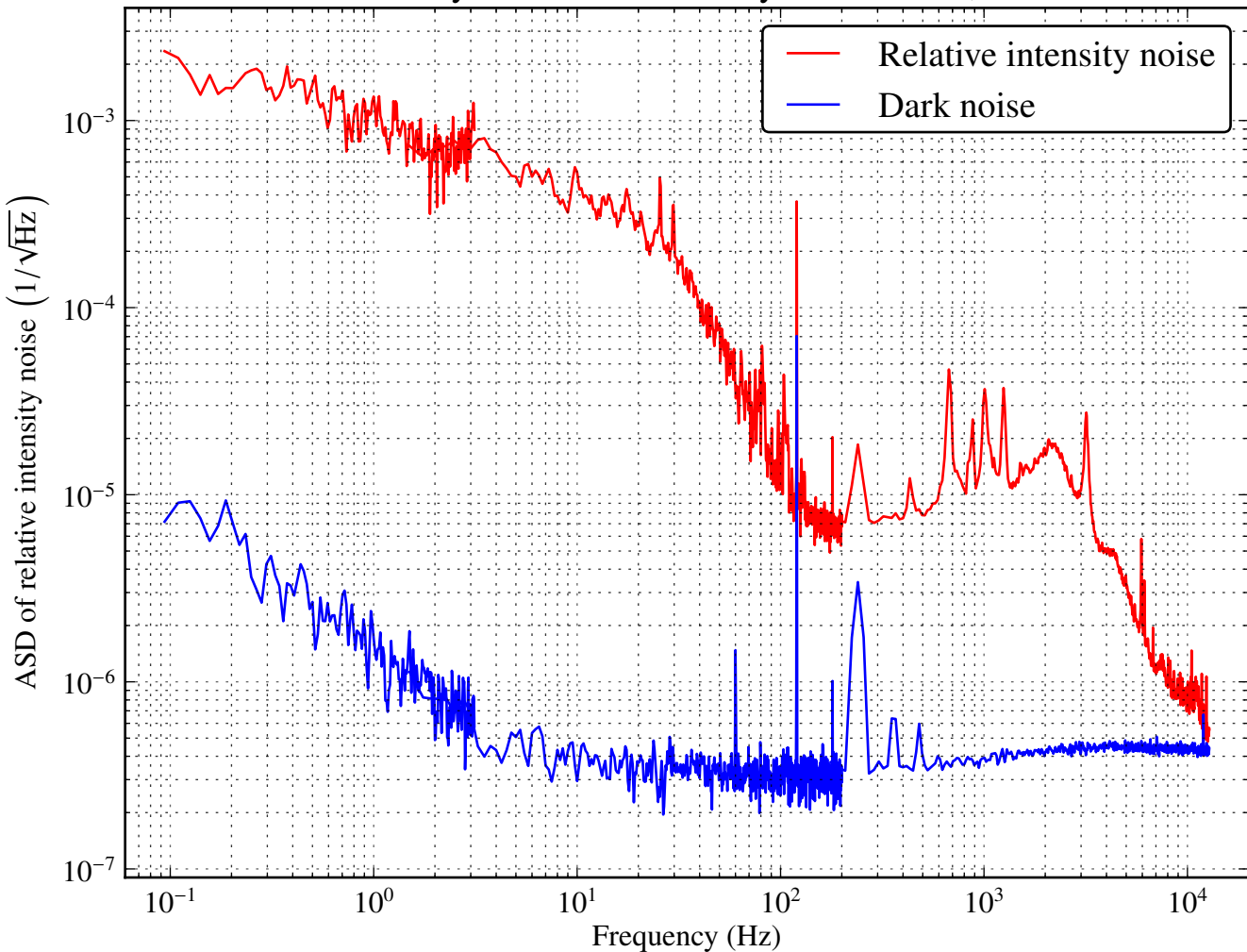
Relative intensity noise of south cavity transmission, 2013-07-29
