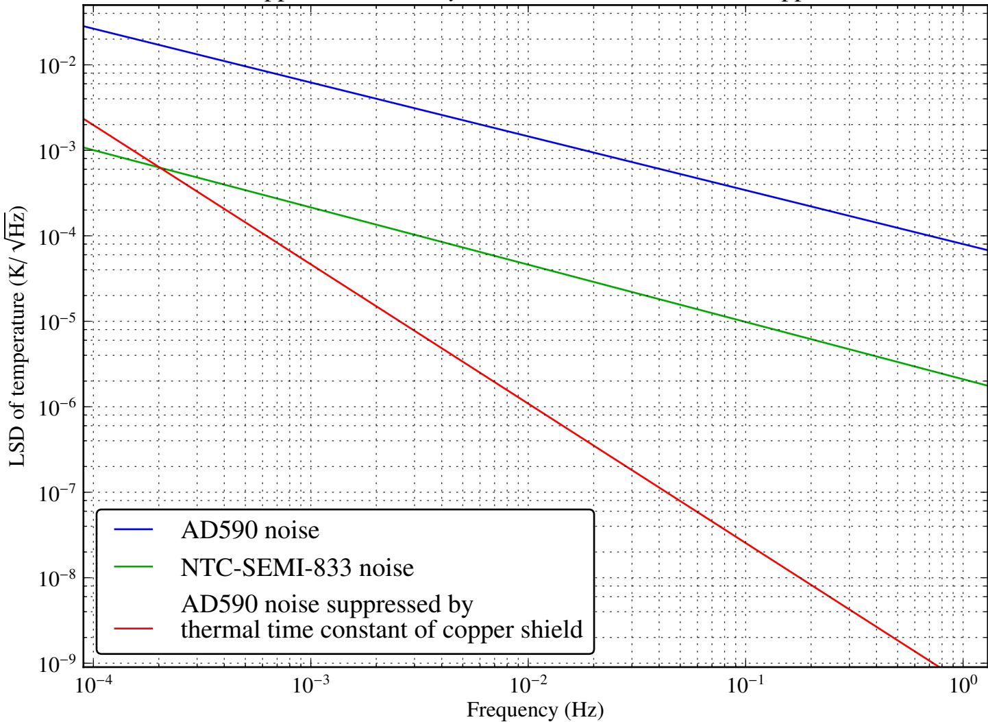
Noise suppression due only to thermal time constant of copper shield
